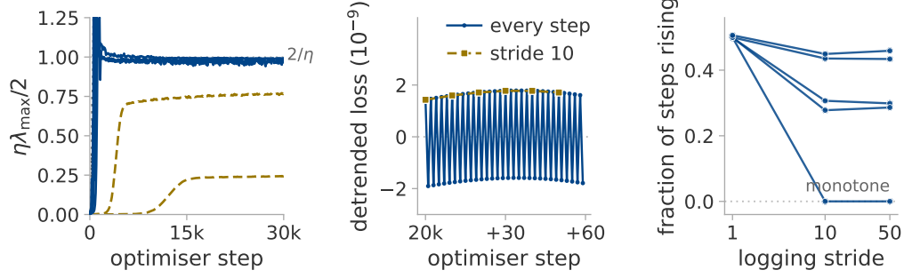
Figure 9: Whether full-batch descent reaches the edge of stability, and the effect of the logging stride. (a) The stability ratio along training, one seed per rate. (b) Sixty consecutive steps at one rate at the edge, against the same series at a stride of ten: the two-cycle is removed by that stride rather than blurred by it. (c) The fraction of steps on which the loss rises, against the logging stride.
