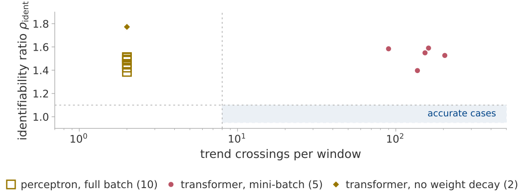
Figure 5: Whether the estimate may be read as a dimension on any grokking log. Every log of section 7 in the plane of the identifiability ratio and the trend-crossing count, the transformer runs observed through the parameter norm and the perceptron runs through the training loss. Colour is the regime of section 3.3, marker shape the setting. The shaded rectangle is where every accurate case of section 6 fell. It is a record of those cases, not a test.
