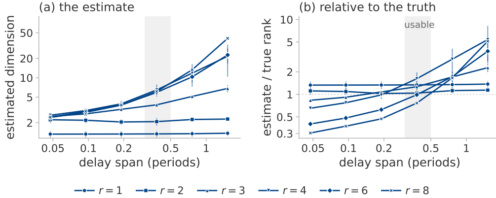
Figure 3: The delay lag, varied on one system: a fixed torus, two seeds, six lags spanning a twentieth of a period to one and a half periods. Marker shape is the true rank, the marker the median of the seeds and the bar their range. (a) The estimate. (b) The same divided by the true rank, so one reference line replaces six; the shaded column is three tenths to a half of a period.
