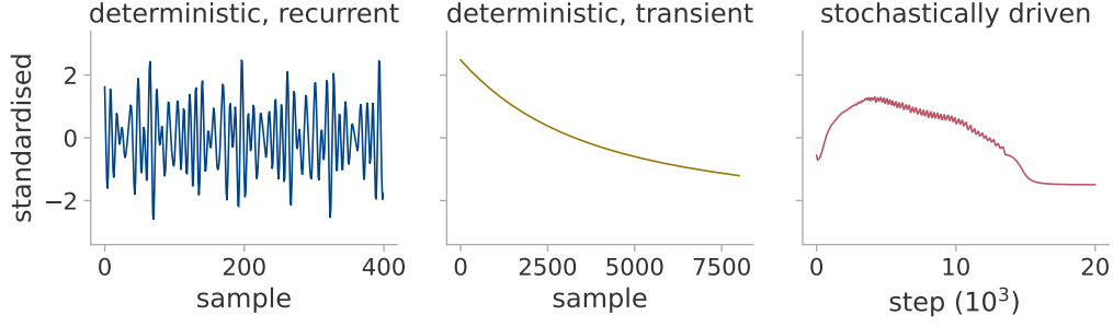
Figure 8: The three regimes as raw scalar logs, standardised to zero mean and unit variance as in Algorithm 1. Left, the constrained head of section 5.2 under a fast quasiperiodic drive, whose path lies on a torus. Middle, the same system under plain gradient descent, which decays over its whole record. Right, a mini-batch transformer run observed through the parameter norm.
