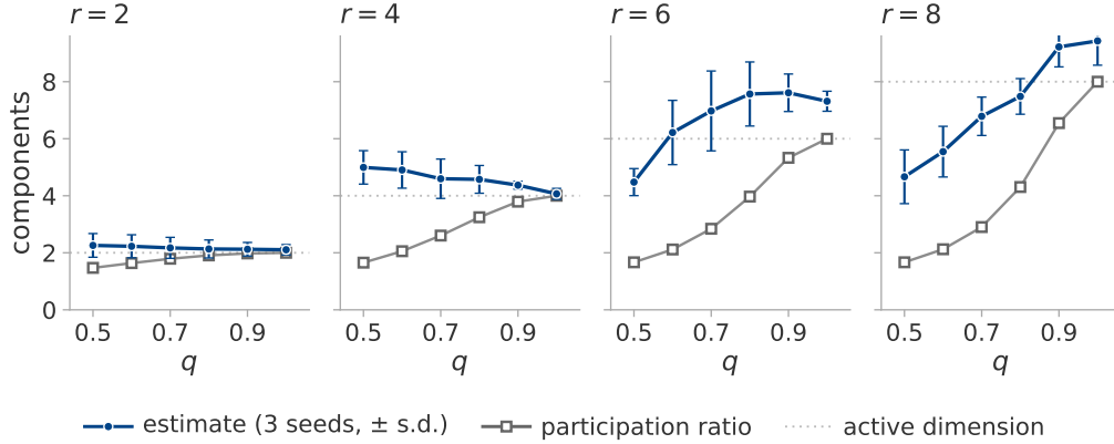
Figure 4: Whether the estimate follows the active dimension or the effective rank. Driving phase l at amplitude q^l holds the active dimension at r while the effective rank falls with q . The system of section 5.1, three seeds, one panel per r ; the dotted line is r . Filled circles, the estimate, median over seeds, with standard deviation as bars; open squares, the measured effective rank, which matches its closed form to two decimals and so has no spread.
