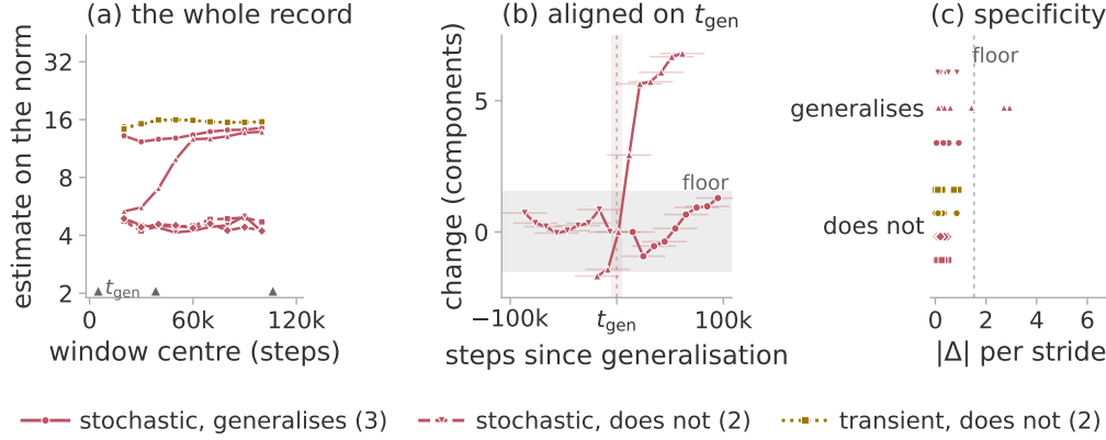
Figure 7: How coarsely a frozen-window estimate localises a feature. The windowed estimate on the parameter norm for the seven extended runs, under the frozen configuration of section 7.1, plotted at the window centres. Colour is the regime of section 3.3. (a) Every window, with the generalisation steps marked on the axis. (b) The generalising runs aligned on their own generalisation step. (c) Every stride-to-stride change, one sub-row per run. The grey band in (b) and (c) is the floor a ramped gain alone produces (section 6.3).
