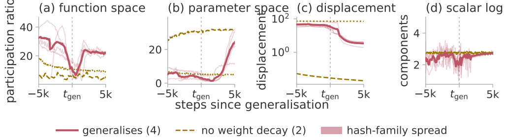
Figure 2: Simplification of the trajectory at generalisation. Three regularised seeds of modular addition and one S_5 composition, against the same two configurations trained without weight decay, aligned on the generalisation step of the run each matches. Thick line, the mean of the four generalising runs; band, the spread between the two hash families (Appendix G.1). Panels (a)–(c) plot \text{PR}^{\text{det}} over windows of 600 steps, 300 for S_5 ; (d) the estimate of section 7.3.
