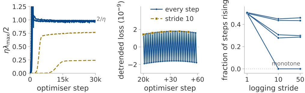
Figure 13: Whether full-batch descent reaches the edge of stability. (a) The stability ratio along training, one seed per rate. (b) Sixty consecutive steps at one rate at the edge, against the same series at a stride of ten: the two-cycle is removed by that stride rather than blurred by it. (c) The fraction of steps on which the loss rises, against the logging stride.
