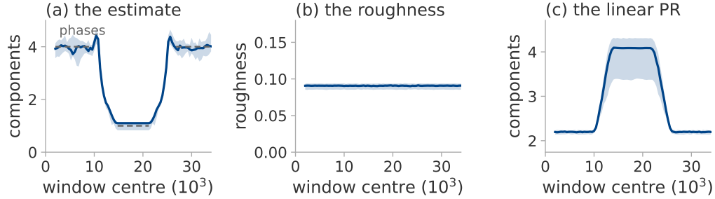
Figure 14: A change in the number of independent phases, tracked as it happens. The harmonic control of this appendix, scheduled from four phases to one and back; median over eight seeds, band their range. Dashed in (a), the number of phases, drawn only where no ramp reaches into the window. Panel (b) is the roughness, which the construction holds fixed; the linear statistic of (c) moves in the opposite direction.
