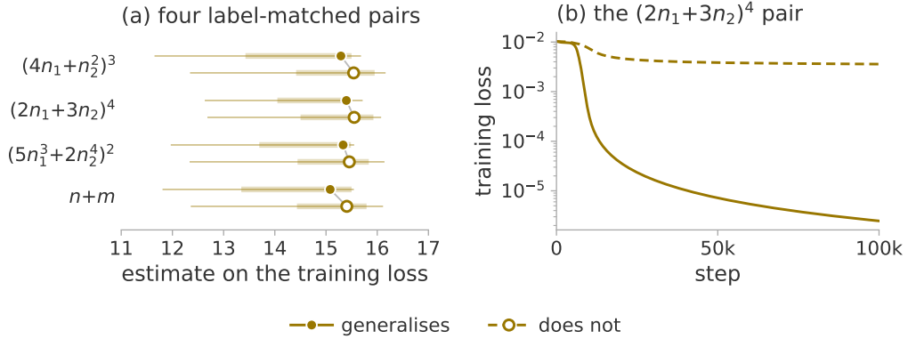
Figure 8: Whether the estimate tells apart two targets that fit the training set alike, only one of them representable by the architecture. (a) The four pairs of section 7.1, on the training loss. Marker, median over the sliding windows; thick bar, interquartile range; thin line, full range. All runs are transient, hence one colour; fill and dash mark generalisation. (b) One pair in full: the representable target drives the loss orders of magnitude lower.
