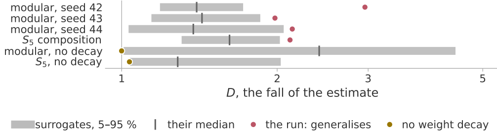
Figure 9: Each run's fall against the null distribution built from that run alone. D is as in table 16, on the parameter-norm log at the headline cell. Band, the fifth to ninety-fifth percentile of the pooled surrogate draws, thirty-nine at each of five seeds; tick, their median; circle, the run. The runs without weight decay are measured in the window of the run each matches.
