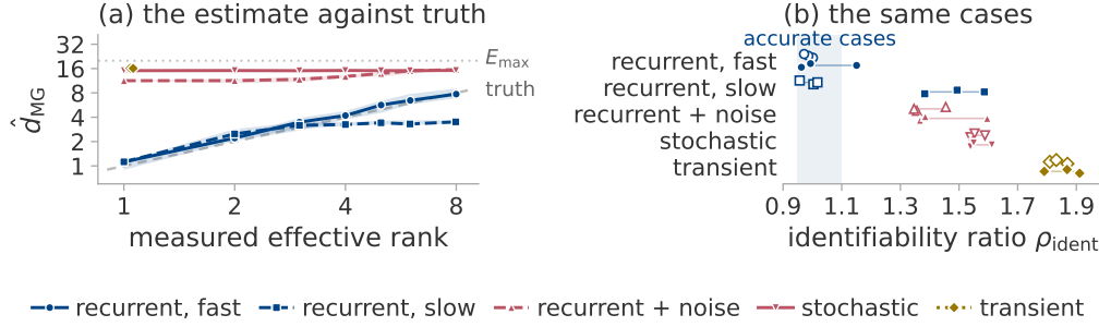
Figure 1: Recovery of the active dimension in each regime. The linear head of section 5.2, driven five ways: recurrent, fast and recurrent, slow quasiperiodic drives, recurrent + noise adding gradient noise to the fast one, stochastic mini-batch noise alone, and transient plain gradient descent. Colour is the regime of section 3.3. (a) Estimate against truth: marker, median over seeds and observers; band, their interquartile range; dashed diagonal, exact recovery; dotted line, E_{\max} . (b) The identifiability ratio on the same five cases, one point per observer, at r = 2 (open) and r = 6 (solid).
