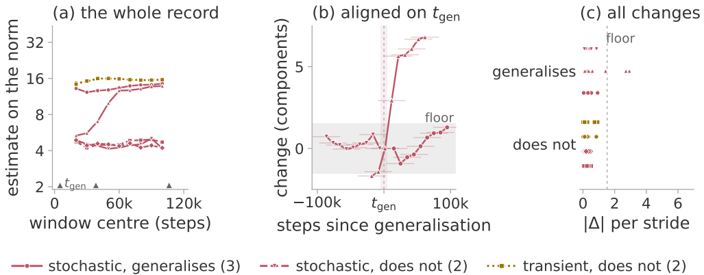
Figure 10: How coarsely a frozen-window estimate localises a feature. The windowed estimate on the parameter norm for the seven extended runs, under the frozen configuration of section 7.1, plotted at the window centres. Colour is the regime of section 3.3. (a) Every window, with the generalisation steps marked on the axis. (b) The generalising runs aligned on their own generalisation step. (c) All the changes from one stride to the next, one sub-row per run. The grey band in (b) and (c) is the floor a ramped gain alone produces (section 6.3).
