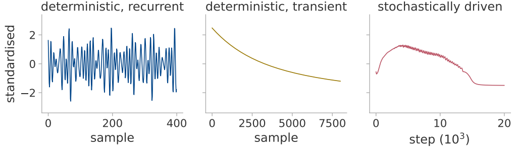
Figure 11: The three regimes as raw scalar logs. Each panel is the parameter norm, standardised to zero mean and unit variance as in Algorithm 1. Left, the constrained head of section 5.2 under a fast quasiperiodic drive, recurrent on a torus. Middle, the same system under plain gradient descent, transient over its whole record. Right, a transformer grokking modular addition, stochastically driven.
