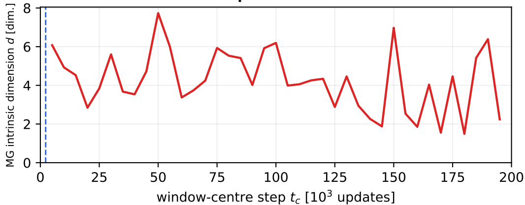
update norm
