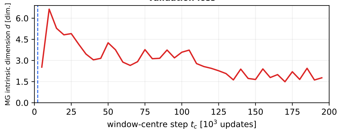
validation loss
