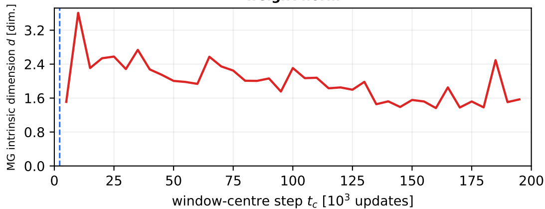
weight norm
