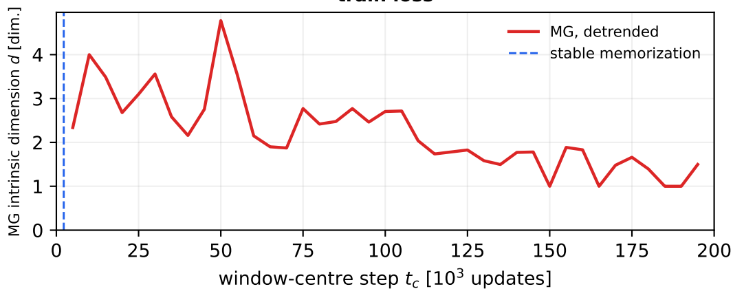
train loss
