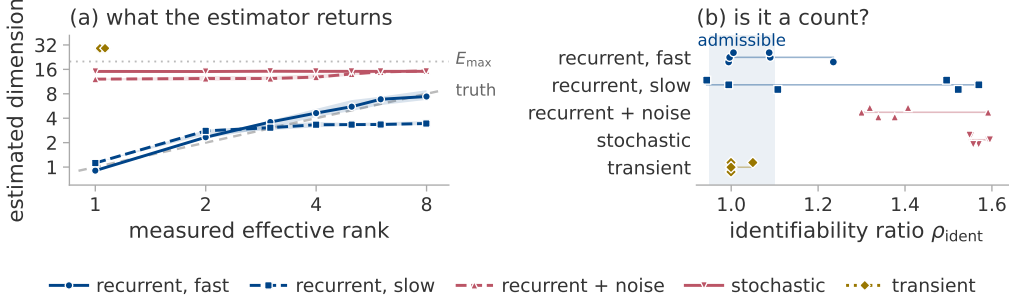
Figure 1: The evaluation of section 5.4: a frozen tanh network on the digits data, a linear head confined to ten directions of which r are excited, five of the nine arms. Colour is the regime of table 1; “fast” and “slow” are the two recurrent drive rates and “+ noise” the fast drive with weak noise added. (a) The estimate against the measured effective rank, which the construction holds at r ; the marker is the median of the forty values behind each point, four seeds by ten observers, and the band their interquartile range. The dashed diagonal is the truth and the dotted line E_{\max} , a reference and not a bound: no clamping is applied and the transient arm sits above it, its seven points piled at x \approx 1.05 because its measured rank is about one at every r . (b) The identifiability ratio, which separates the regimes with no ground truth; the shaded column is the admissible band. It is not computed on the runs of (a): the sweep populates it for seed 0, three observers and r \in \{2, 6\} only, so each regime rests on the six values plotted. The transient is the one regime it passes, hence the trend-crossing count of section 3.4.
