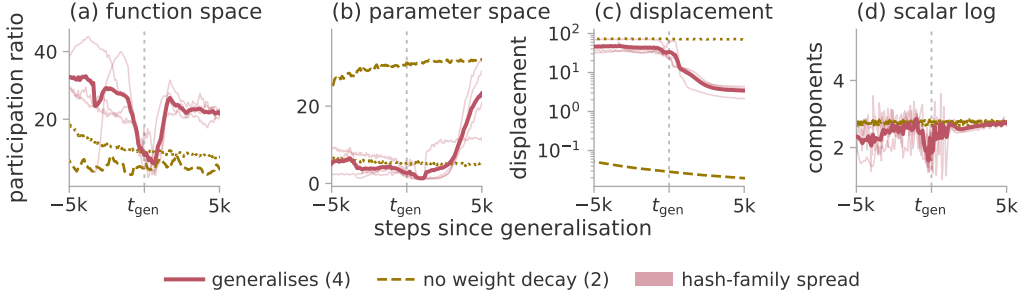
Figure 2: Three seeds of modular addition at weight decay 1.0 and one S_5 composition at 0.2, against the same two configurations at weight decay zero, which memorise and stay at chance accuracy. Colour is the regime of table 1, so the four regularised runs are stochastic and the two controls transient; the thick line is the mean of the four that generalise, and each control is aligned on the generalisation step of its matched run. The statistic in (a)–(c) is \text{PR}^{\text{det}} , an effective rank: these runs have no recurrent set, so no active dimension is defined for them. Its windows are 600 optimiser steps for the modular runs and 300 for S_5 , at their midpoint, so a feature is located to within \pm 300 and \pm 150 steps; the band on (a) and (b) is the two-hash disagreement, under two per cent of the mean (Appendix I). Panel (d) is a different measurement on the same midpoints: the delay estimate of section 7.3 on the parameter-norm log, at a 600-step window.
