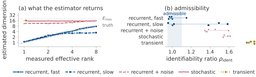
Figure 1: Recovery of the active dimension in each regime, and separation of the regimes without ground truth. Five of the nine excitation cases of section 5.4; colour is the regime of table 1. (a) The estimate against the measured effective rank, which the construction holds at r ; the marker is a median over four seeds and ten observers, the band their interquartile range, the dashed diagonal the truth. The dotted line is E_{\max} , a reference and not a bound. (b) The identifiability ratio, on a smaller grid; the transient is the one regime it passes.
