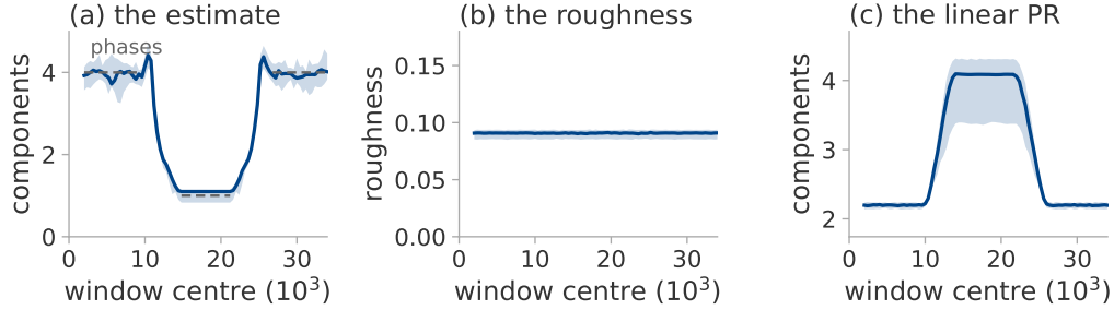
Figure 13: A change in the number of independent phases, tracked as it happens. The harmonic control of this appendix, scheduled from four phases to one and back; median over eight seeds, band their range. Dashed in (a), the number of phases, drawn only where no ramp reaches into the window. The linear statistic of (c) moves in the opposite direction.
