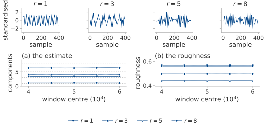
Figure 4: The log the estimator is given and the level it returns. The image-data system of section 5.2 at four ranks and a seed the configuration was not selected on, observed through the parameter norm. Above, four hundred samples of each log. (a) The estimate over sliding windows, with the measured effective rank dotted. (b) The roughness of the same windows.
