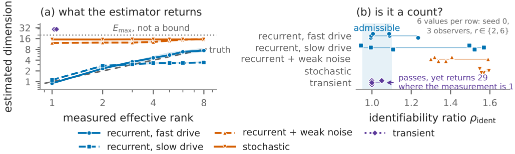
Figure 1: The evaluation of section 5.4: a frozen tanh network on the digits data, a linear head confined to ten directions of which r are excited, five of the nine arms. (a) The estimate against the measured effective rank, which the construction holds at r ; the marker is the median of the forty values behind each point, four seeds by ten observers, and the band their interquartile range. It tracks the truth only under a fast recurrent drive. The seven transient points pile up at x \approx 1.05 because that arm’s measured rank is about one at every nominal r ; that is the measurement, not missing data. (b) The identifiability ratio, which separates the regimes with no ground truth. It is not computed on the runs of (a): the sweep populates it for seed 0, three observers and r \in \{2, 6\} only, so each regime rests on the six values plotted, one sub-row per observer. The transient is the one regime it passes, hence the trend-crossing count of section 3.4.
