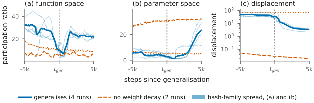
Figure 2: The trajectory effective rank measured directly, on three seeds of modular addition at weight decay 1.0 and one S_5 composition at 0.2, against the same two configurations at weight decay zero, which memorise and stay at chance validation accuracy. The statistic is \text{PR}^{\text{det}} of section 3.1, an effective rank: these runs have no recurrent set, so no active dimension is defined for them. Windows are 600 optimiser steps for the modular runs and 300 for S_5 , at their midpoint, so a feature is located to within \pm 300 and \pm 150 steps; each control is aligned on the generalisation step of its matched run, and the band on (a) and (b) is the two-hash disagreement, under two per cent of the mean (Appendix I).
