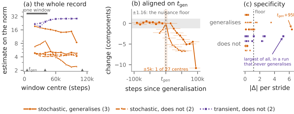
Figure 5: The windowed estimate on the parameter norm for the seven extended 120 000-step runs, under the frozen configuration of section 7.1: nine windows per run of 39 990 optimiser steps each, advanced by 10 000, plotted at their centres. Colour is the regime of table 1, five runs stochastic and two transient, none recurrent. (a) All sixty-three windows, with the three generalisation steps marked and one window drawn to scale in grey. (b) The three generalising runs aligned on their own generalisation step, each point a change from the window before it and its bar the span it summarises, so consecutive points share three quarters of their span. The grey band is the \pm 1.16 -component floor of section 6.3 and the shaded column is \pm 5 000 steps of t_{gen} , which one of the twenty-seven centres reaches. (c) Every stride-to-stride change, one sub-row per run so that coincident changes stay countable. The largest in the set is in a run that never generalises.
