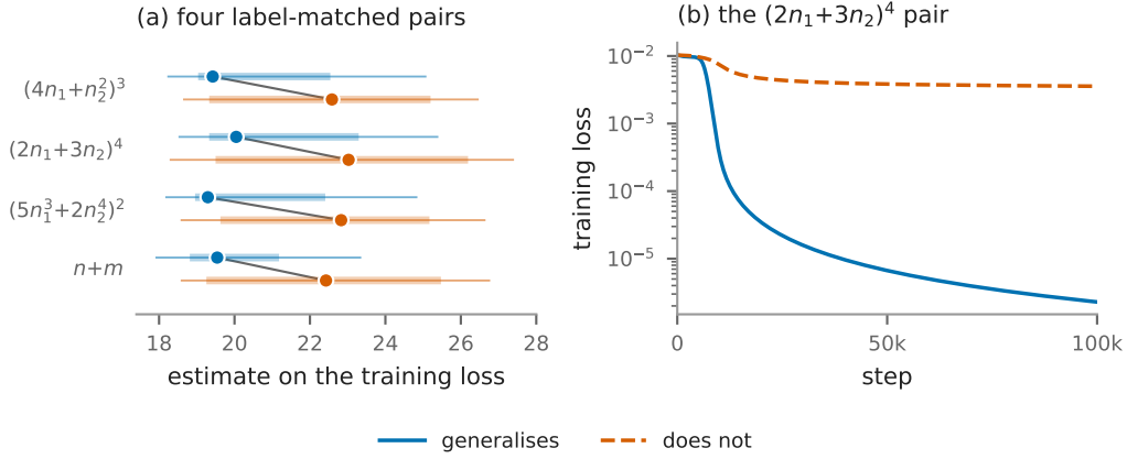
Figure 4: (a) The estimate on the training loss for the four label-matched pairs of section 7.2: three modular polynomials at p = 97 , each against itself perturbed by one monomial, and modular addition against n^3 + nm^2 + m . Both members of a pair reach full training accuracy under identical optimisation on identical data budgets. The marker is the median over the seven sliding windows, the thick bar their interquartile range and the thin line their full range. The medians separate the two members of every pair, by 2.88 to 3.54 units and with no overlap between the two groups of medians, but the window-level ranges overlap heavily, because the estimate drifts upward over training in every run rather than scattering about a level. (b) The (2n_1+3n_2)^4 pair, the second row of (a). The representable target drives the training loss to 2.3 \times 10^{-6} while the perturbed one stops at 3.6 \times 10^{-3} , three orders of magnitude short despite fitting the training set completely, so the two curves differ in shape rather than in any attractor dimension. Across the four pairs that gap runs from 2.7 to 3.2 orders.
