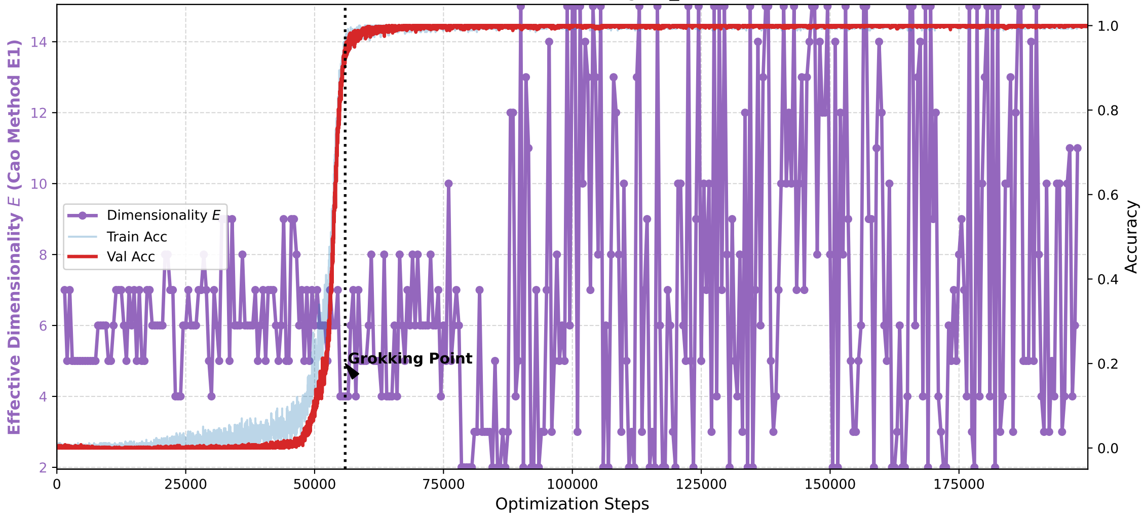
Collapse of Dimensionality during Grokking Method: Cao Method E1 (Metric: grad_cosine, W=300)
