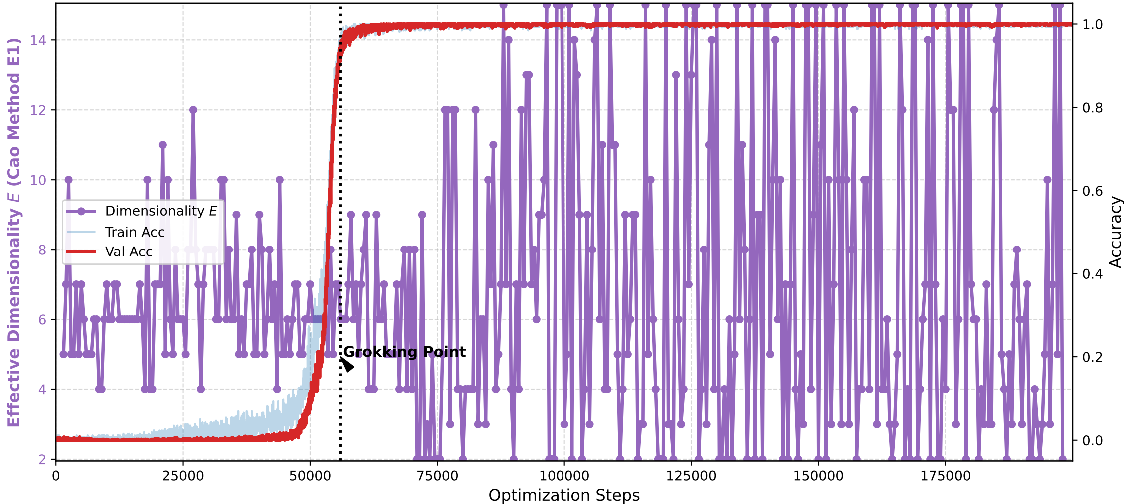
Collapse of Dimensionality during Grokking Method: Cao Method E1 (Metric: grad_norm, W=300)
