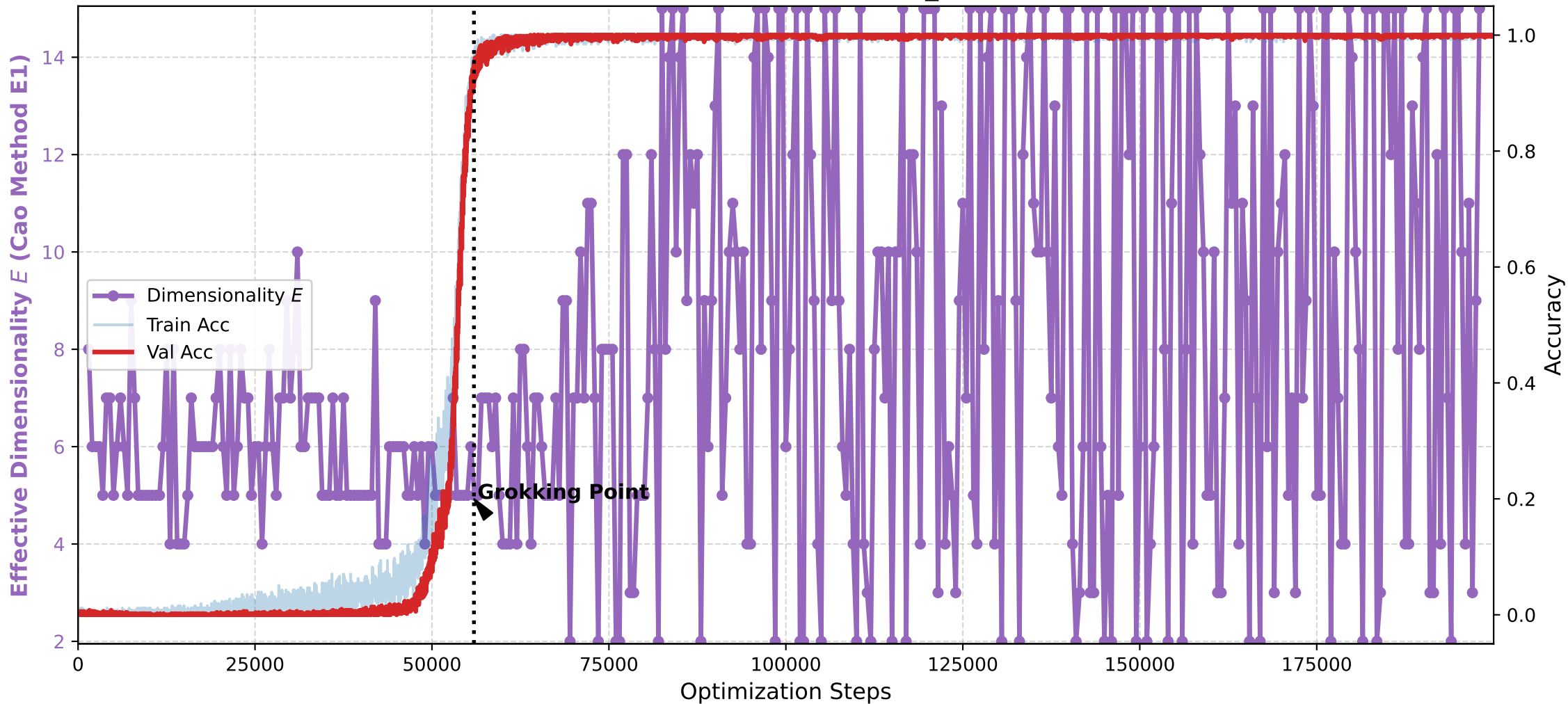
Collapse of Dimensionality during Grokking Method: Cao Method E1 (Metric: val_loss, W=300)
