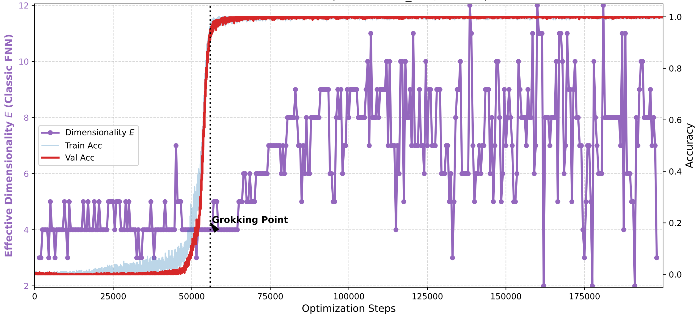
Collapse of Dimensionality during Grokking Method: Classic FNN (Metric: train_loss, W=300)
