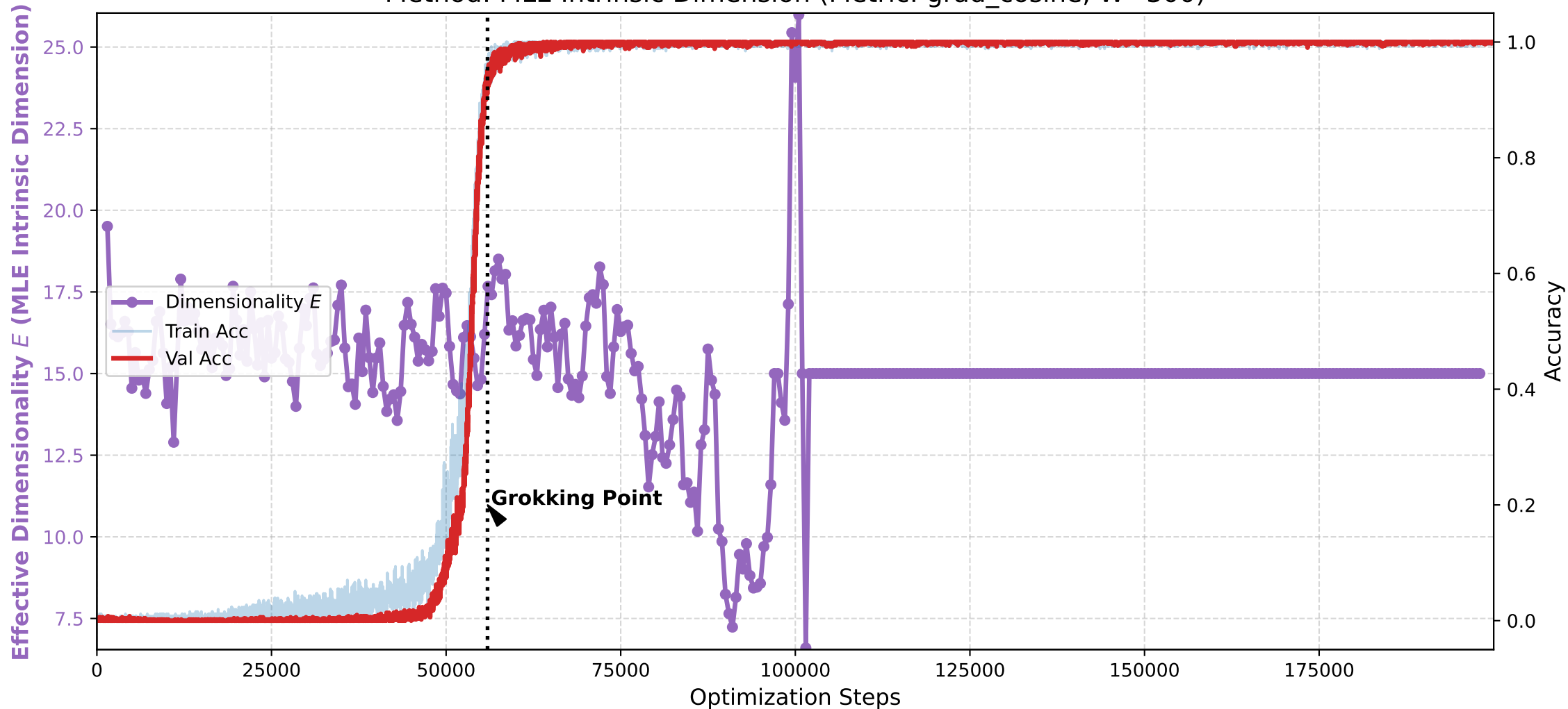
Collapse of Dimensionality during Grokking Method: MLE Intrinsic Dimension (Metric: grad_cosine, W=300)
