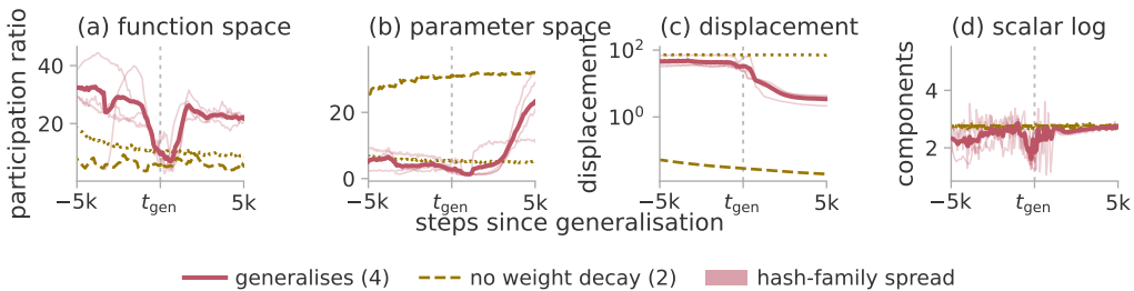
Figure 2: Simplification of the trajectory at generalisation, measured against two controls. Three regularised seeds of modular addition and one S_5 composition, against the same two configurations without weight decay, which memorise and stay at chance accuracy. Colour is the regime of table 1; the thick line is the mean of the four runs that generalise, and each control is aligned on the generalisation step of its matched run. The statistic in (a)–(c) is \text{PR}^{\text{det}} , an effective rank: none of these runs recurs, so none supports reading a dimension. Windows are 600 optimiser steps, 300 for S_5 , plotted at their midpoint; the band on (a) and (b) is the two-hash disagreement (Appendix I). Panel (d) is a different measurement on the same midpoints: the delay estimate of section 7.3 on the parameter-norm log.
