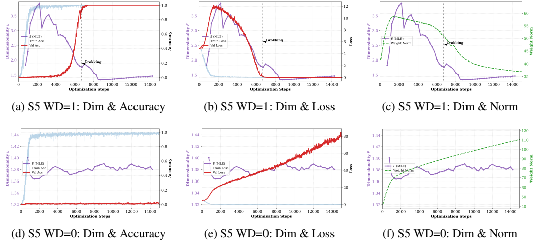
Рис. 2: Analysis of composition in the S_5 group. The dimensionality collapse reliably captures the structural reorganization of the network, even for the complex multidimensional topology of a non-abelian group.
