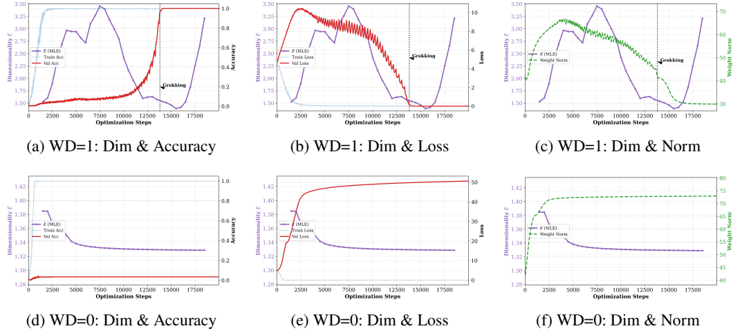
Рис. 1: Analysis of grokking on modular addition in the presence of stochastic noise. The plots compare the dynamics of dimensionality E (derived from the weight norm series) against Accuracy, Loss, and Weight Norm in regimes with generalization (top row) and without it (bottom row).
