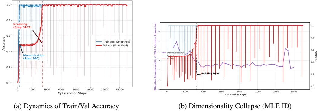
Рис. 4: The grokking phenomenon in the baseline experiment (Full-Batch). The transition from memorization to generalization is accompanied by a decrease in the topological complexity of the \mathcal{L}_{train} trajectory; however, the estimation suffers from a lack of variance due to the degeneration of the series.
