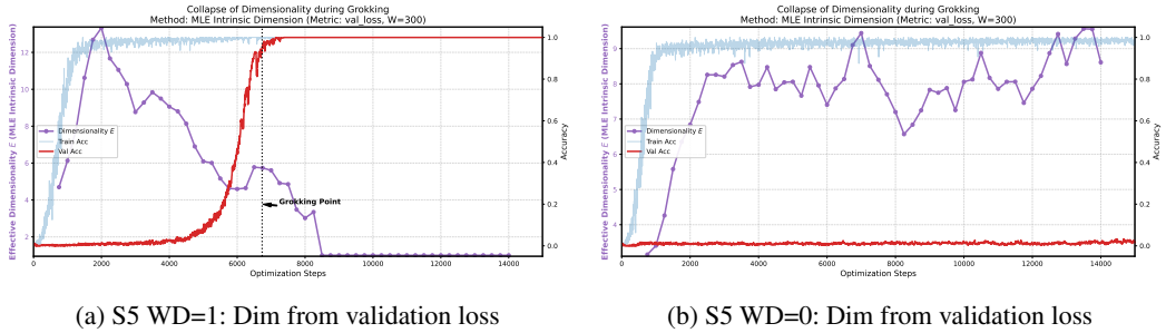
Рис. 3: Analysis of the S_5 group. The dimensionality E reconstructed from the validation loss successfully estimates the true algebraic complexity of the algorithm (plateauing at \hat{d} \approx 4 ).
