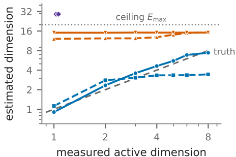
(a) what the estimator returns
