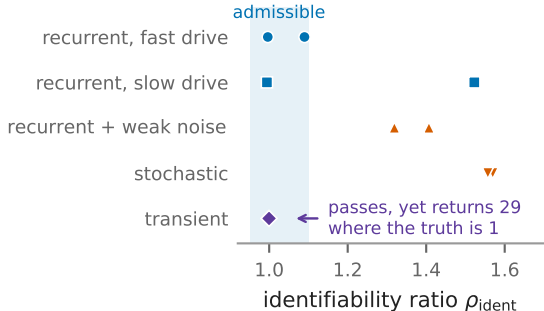
(b) is it a count?
