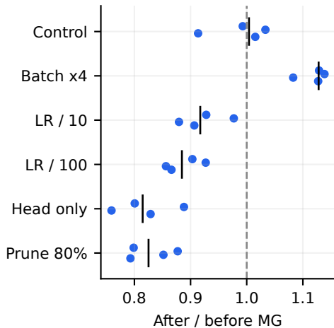
CNN: new seeds
