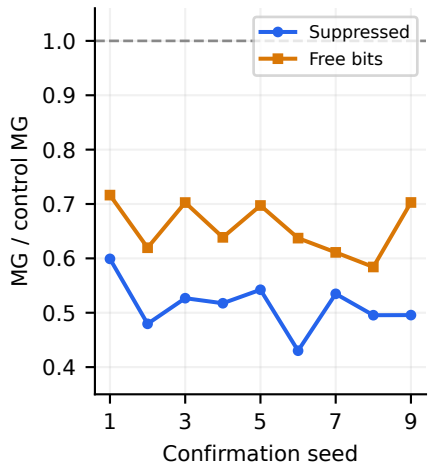
VAE: paired branches
