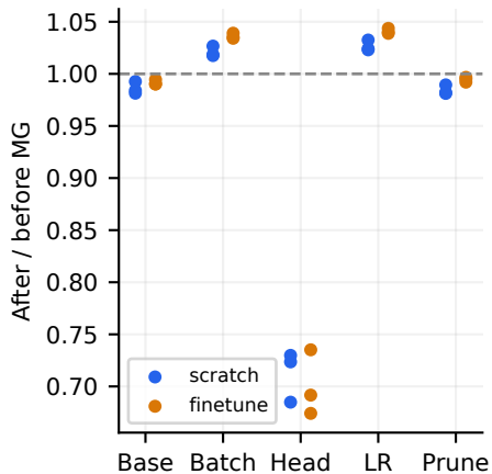
ResNet: frozen rule
