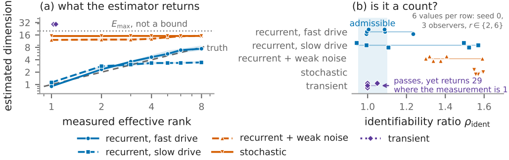
Figure 1: The evaluation of section 5.4: a tanh network trained on sklearn digits and frozen, a linear head confined to ten directions of which r are excited, five excitation regimes. (a) The estimate against the measured effective rank, which the construction holds at r , median over four seeds and ten observers; it tracks the truth only under a fast deterministic recurrent drive. (b) The identifiability ratio on the same runs, which separates those regimes without a ground truth. The transient is the one regime it passes, hence the recurrence count of section 3.4.
