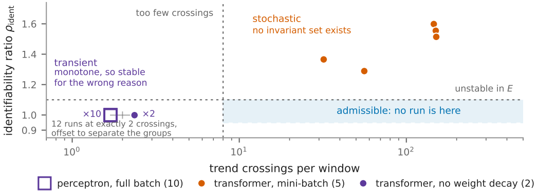
Figure 2: Every training log of this section in the plane of the two diagnostics of section 3.4, one point per run: seven transformer runs of 120 000 steps observed through the parameter norm, and ten perceptron runs of 100 000 steps observed through the training loss. The vertical axis is the identifiability ratio, near unity when the estimate does not depend on the embedding dimension; the horizontal axis counts how often the series crosses its own least-squares line inside a window. The shaded rectangle is where every accurate case of section 6 fell: \rho_{\text{ident}} \leq 1.10 , which is the top of the range observed on the recurrent arms, and more than eight crossings, which is the bottom of the range on any arm the estimate tracked. It is a description of the calibration, not a validated decision rule, and no run of either setting is inside it. The two settings fail in different corners, and both failures are visible without any label.
