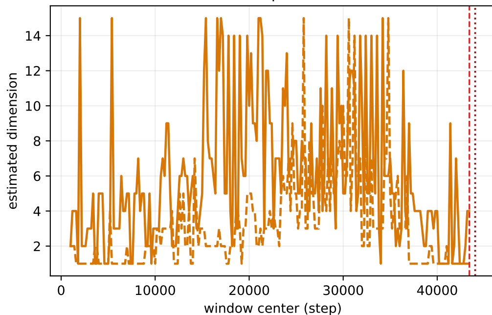
Simplex
