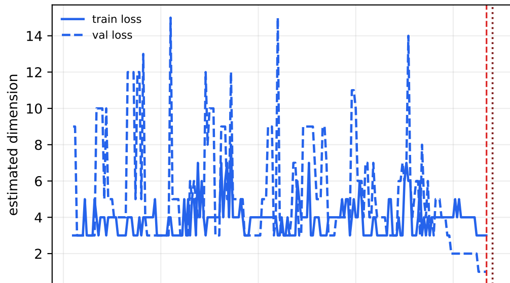
FNN
