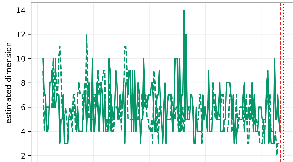
Cao
