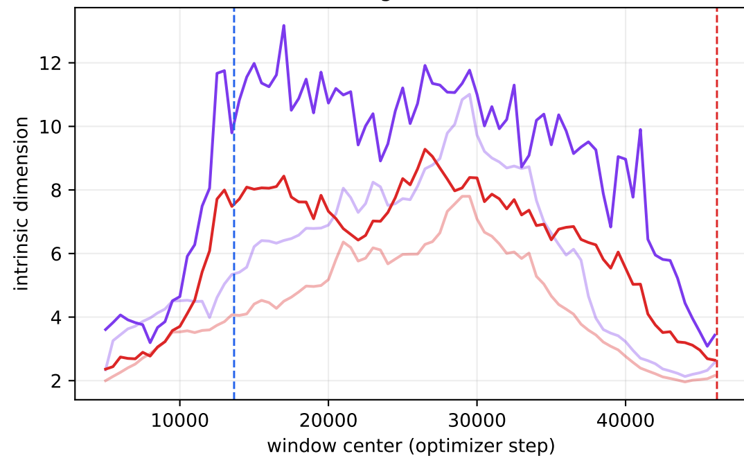
weight norm
