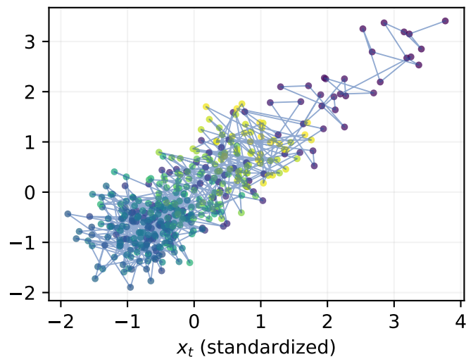
detrended: x_{t+\tau}
