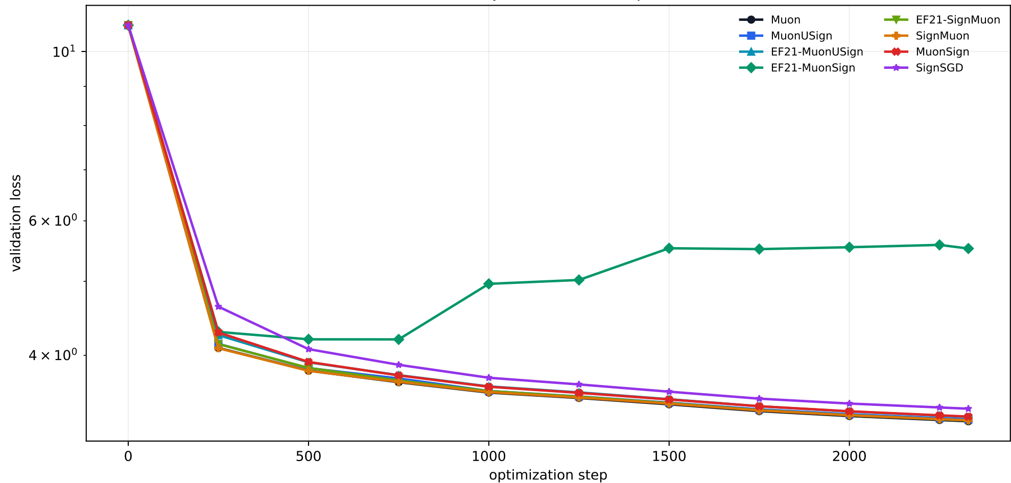
Validation trajectories across optimizers
