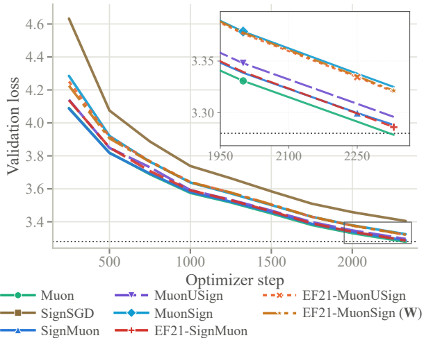
Figure 3: NanoGPT speedrun, 8\times H100 : validation loss against optimizer step, one run per method; dotted is the target 3.28, and EF21-MuonSign is drawn at its broadcast model W . The inset magnifies the boxed tail, where SignSGD lies above the range shown.
