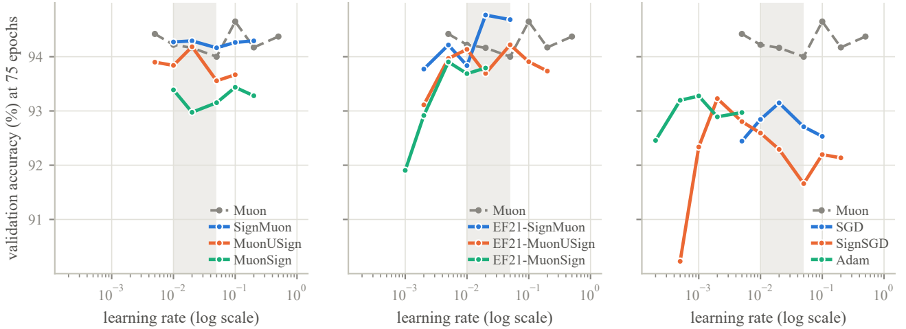
Figure 9: Learning-rate sweep at the 75-epoch selection horizon, on the tuning split and on the validation accuracy that selection ranked, grouped as in Figure 2, with Muon repeated as the gray dashed reference. The shaded band marks \eta_0 \in [0.01, 0.05] , the only interval every method but Adam was swept over; the nine vary by 0.10 to 0.93 points within it, SGD (0.44) among them, so an absolute window no longer discriminates between the families, their optima lying two decades apart. The matched comparison is the relative one. Within a factor of five of its own optimum SignMuon varies by 0.13 points and SignSGD by 3.00; the two emit steps of identical Frobenius length, so the difference is attributable to the LMO. The remaining eight lie between these, from 0.46 (MuonSign) to 2.00 (EF21-MuonSign). Taking the sign of the oracle’s output does not reduce this insensitivity: SignMuon’s sweep is the flattest of the ten.
