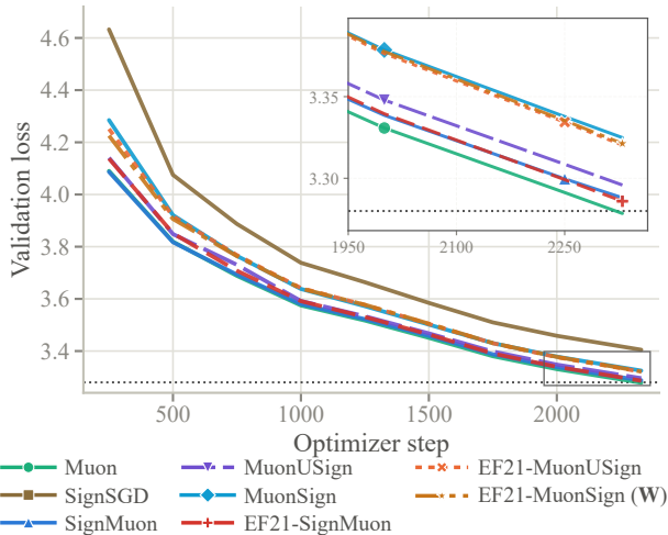
Figure 3: NanoGPT speedrun, 8\times H100 : validation loss against optimizer step, single seed; dotted line is the speedrun target 3.28. EF21-MuonSign is drawn at its broadcast model W . The inset magnifies the boxed tail, where SignSGD is above the range shown; exact values are in Table 3.
