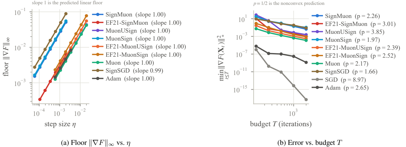
Figure 5: Log-log fits behind Table 7. Left: the accuracy floor of a constant step; the lines are parallel because every exponent is 1, and the two clusters are the two step lengths, \|\mathbf{S}\|_F = \sqrt{mn} on the left and \sqrt{r} on the right. Right: best error at each tuned budget, in the norm dual to each method’s own LMO ball, so the curves are comparable within a family and not across one.
