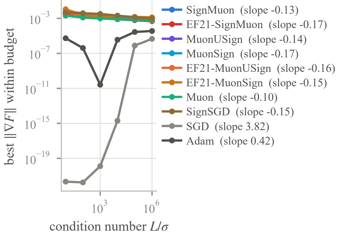
Figure 6: Best \|\nabla F\| within the budget against the condition number L/\sigma , tuned at each point. The eight norm-fixed methods lie in a band an order of magnitude wide and essentially flat; SGD and Adam are the two that resolve the sweep at all.
