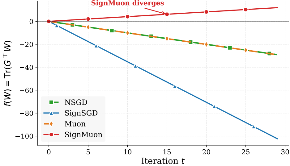
Figure 1: Comparison of optimization trajectories for the linear objective function f(\mathbf{W}) = \text{Tr}(\mathbf{G}^\top \mathbf{W}) , demonstrating the strict divergence of SignMuon, while other methods successfully minimize the function.
