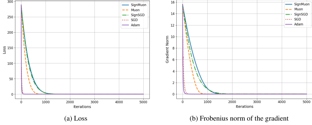
Figure 2: Smooth convex problem (Equation 11 for 500 \times 500 ).
