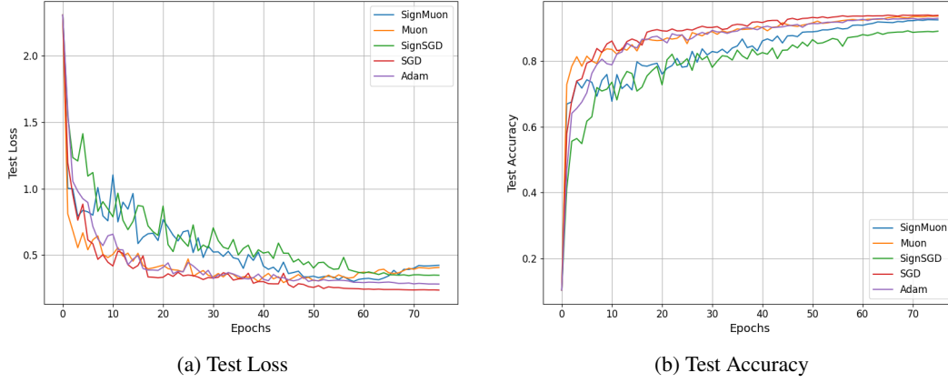
Figure 4: Centralized setting. Comparison of convergence and classification accuracy achieved by different optimization algorithms during CIFAR-10 classifier training on the test set.
