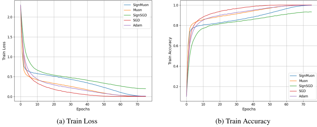
Figure 3: Centralized setting. Comparison of convergence and classification accuracy achieved by different optimization algorithms during CIFAR-10 classifier training on the training set.
