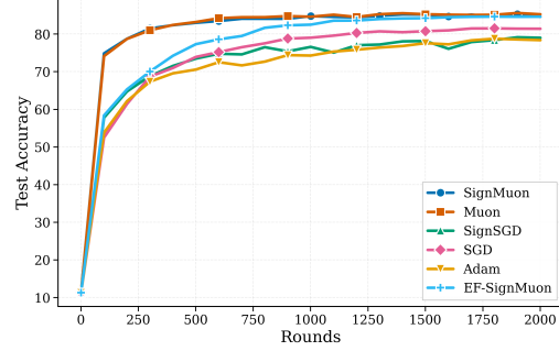
(b) Test Accuracy
