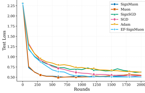
(a) Test Loss
