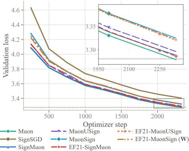
Figure 3: NanoGPT speedrun, 8\times H100 : validation loss against optimizer step, single seed; dotted is the target 3.28, and EF21-MuonSign is drawn at its broadcast model W . The inset magnifies the boxed tail, where SignSGD lies above the range shown.
