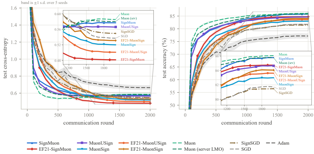
Figure 11: CIFAR-10 federated learning on CNN2 at N = 11 clients and batch 192 per client, every method evaluated on the exact server model \mathbf{X}_t . Both panels are clipped to exclude round 0, the untrained model, which is identical for every method. Solid lines are the one-bit methods, dashed the uncompressed references and dash-dot SignSGD, so that hue is not the only channel separating eleven curves. The insets magnify the final 45% of rounds, where every number in Table 1 is read, and name each curve at its own end; Adam finishes clear of the other ten and so falls outside the magnified window. Eleven methods are drawn, one more than Table 1, the extra being the server-side-LMO Muon control.
