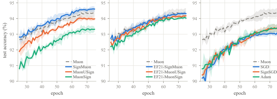
Figure 2: Centralized ResNet-18 on CIFAR-10: test accuracy from epoch 25 at each method’s selected \eta_0 (Table 2). Panels group the sign placements, the EF21 variants and the baselines; Muon is the gray dashed reference, bands \pm 1 s.d. over three seeds. The numbers are Table 2, Appendix A.4.
