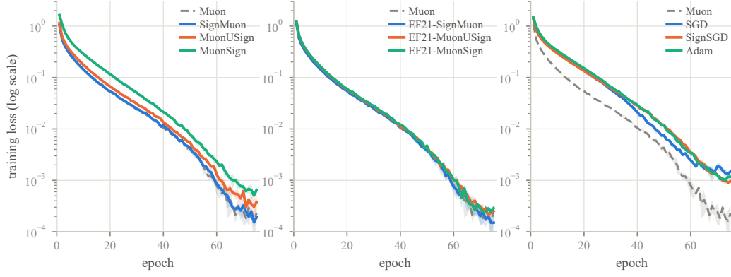
Figure 9: Training loss (log scale), grouped as in Figure 2 and over the same runs. Within a panel the methods are hard to separate (eight of the ten fall below 10^{-3} , differing mainly in how early), which is why the body figure carries the accuracy alone. What the loss does show is the separation between families: in the right panel Muon reaches 10^{-2} six to eleven epochs before SGD, SignSGD and Adam and terminates four to six times lower, while in the left panel SignMuon tracks Muon and the sign-before and both-sides orderings lie above it, in the same order as their accuracies. The three EF21 variants (centre) are indistinguishable in loss, whereas their accuracies span 0.27 points.
