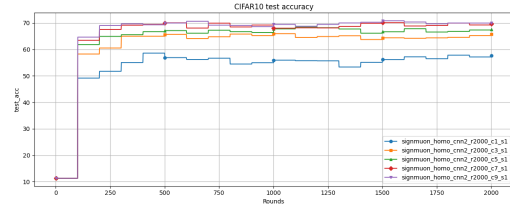
(b) Test Accuracy
