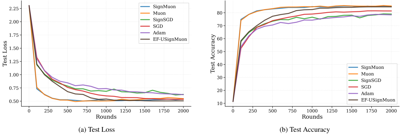
Figure 7: CIFAR-10 Federated Learning on CNN2. Experiment 2: Comparison of Optimization Algorithms with (N = 10) Clients.
