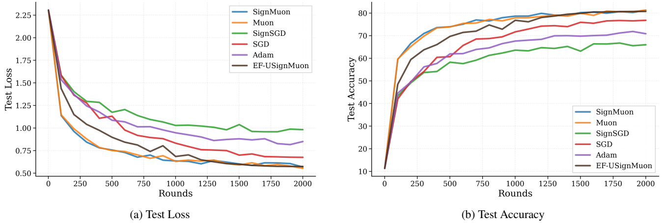
Figure 6: CIFAR-10 Federated Learning on CNN2. Experiment 1: Comparison of Optimization Algorithms with (N = 3) Clients.
