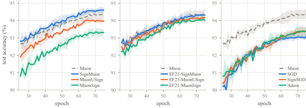
Figure 2: Centralized ResNet-18 on CIFAR-10: test accuracy from epoch 25 at each method’s selected \eta_0 (Table 2). Panels group the sign placements, the EF21 variants and the baselines; Muon is the gray dashed reference, bands \pm 1 s.d. over three seeds. The numbers are Table 2, Appendix A.4.
