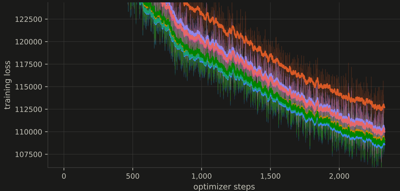
NanoGPT speedrun (record #40): training loss vs steps
