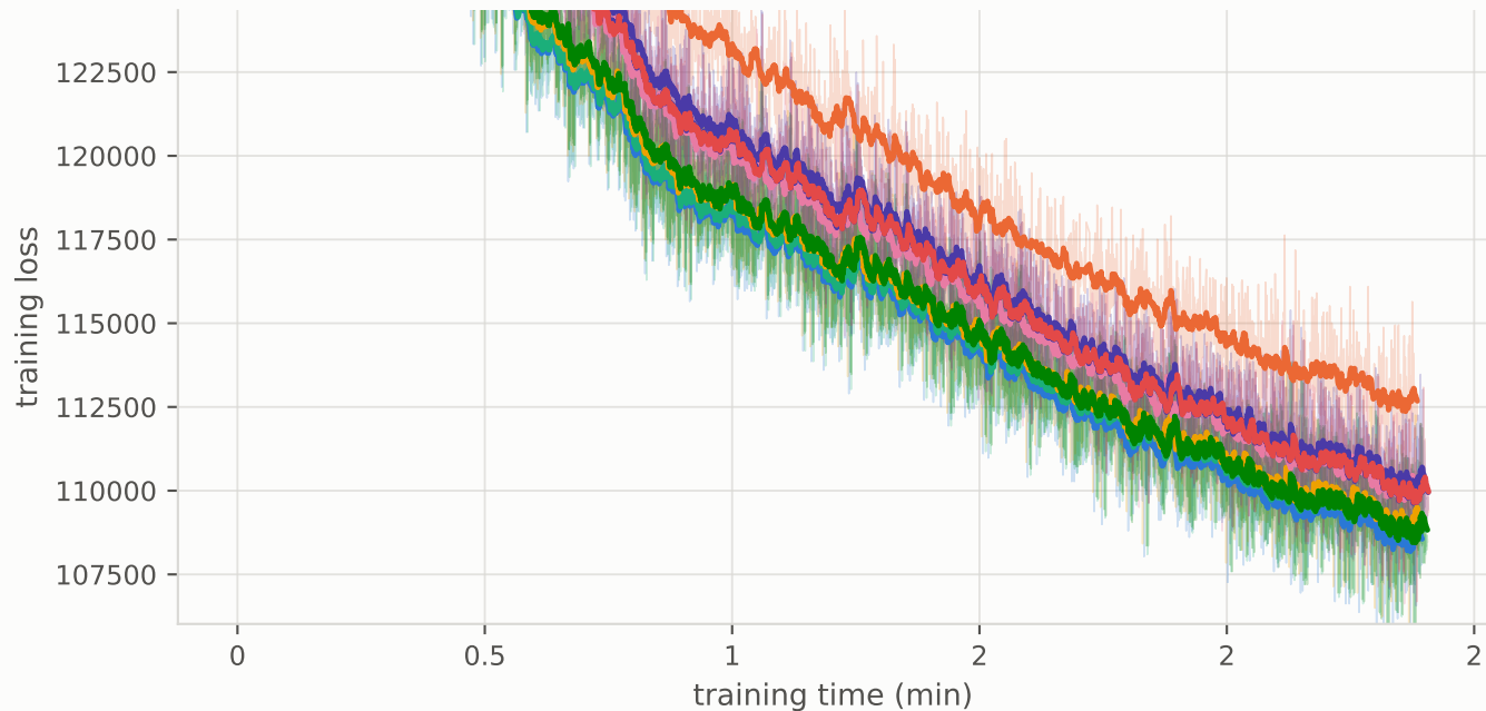
NanoGPT speedrun (record #40): training loss vs wall-clock
