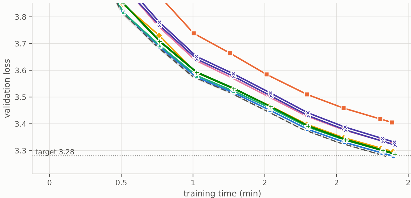
NanoGPT speedrun (record #40): validation loss vs wall-clock
