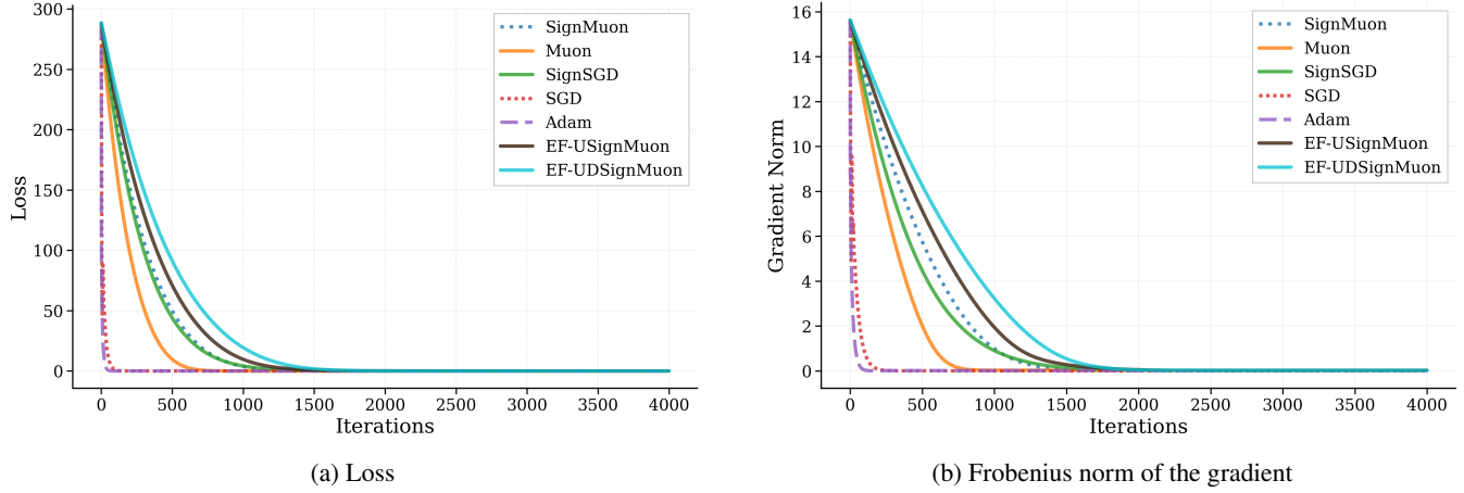
Figure 3: Smooth convex problem (Equation 12 for 500 \times 500 ).
