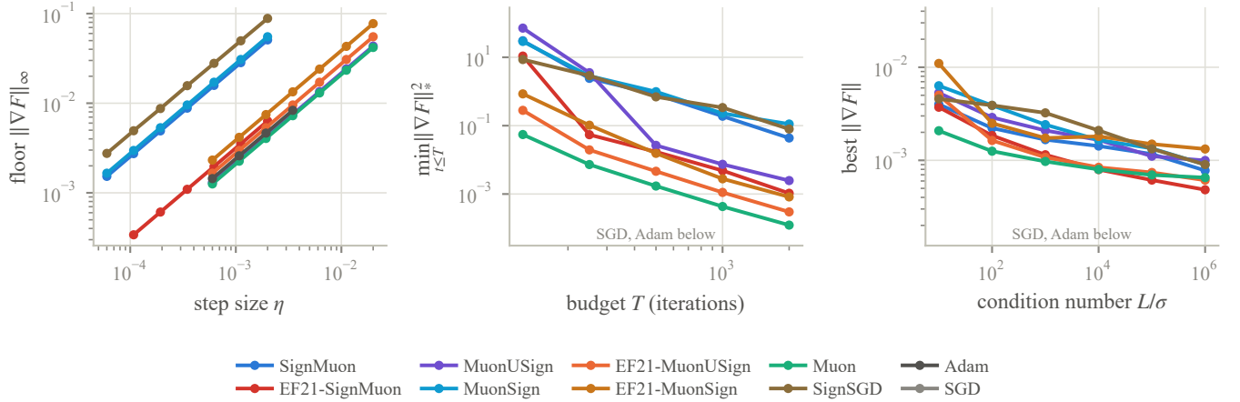
Figure 6: Log–log fits behind Table 8, at m = n = 100 over three problem draws. Left , the accuracy floor of a constant step: the lines are parallel because every exponent is 1, and the two clusters are the two windows of \eta swept, one per step length. EF21-SignMuon falls in the left cluster although its step has length \sqrt{r} , having been swept over the sign family’s window; the misassignment displaces the line along \eta without altering its slope (see Protocol ). Centre , best error at each tuned budget, in the norm dual to each method’s own LMO ball, hence comparable within a family but not across families. Right , best \|\nabla F\| within the budget against L/\sigma , tuned at each point; the eight norm-fixed methods are flat in \kappa to within a factor of three. In the last two panels the vertical range is set by those eight methods, and SGD and Adam leave the frame below: on a quadratic with an exactly known Hessian a scaled gradient step converges to machine precision, fifteen decades below anything with a norm-fixed step, and on a shared range the eight would occupy a single line.
