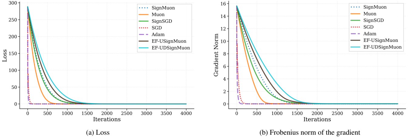
Figure 7: Smooth convex problem (Equation 45 for 500 \times 500 ).
