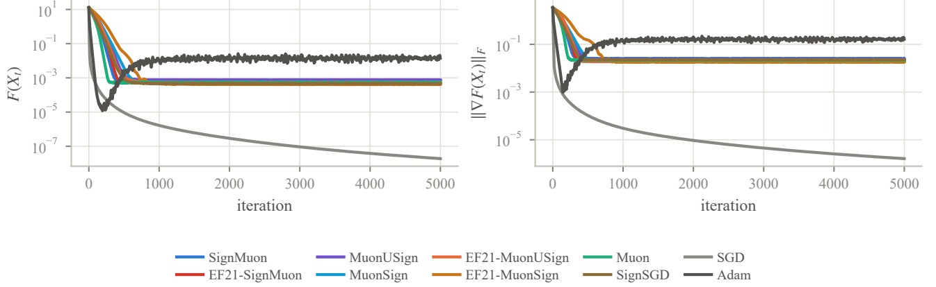
Figure 5: Trajectories at the optima of Table 6, mean over three problem draws. Every normalized method reaches a plateau within a few hundred iterations and remains there, which is what makes the crossing time a ranking of floors. SGD, whose step vanishes with the gradient, is the only curve still descending at T_{\max} ; Adam oscillates about its floor rather than settling onto it.
