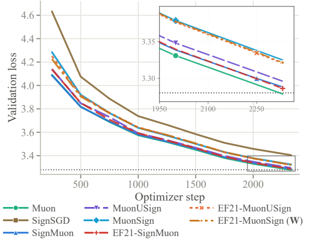
Figure 3: NanoGPT speedrun, 8 \times H100 : validation loss against optimizer step, single seed; dotted is the speedrun target 3.28. EF21-MuonSign is drawn at its broadcast model W . The inset magnifies the boxed tail, where SignSGD is above the range shown; exact values are in Table 3.
