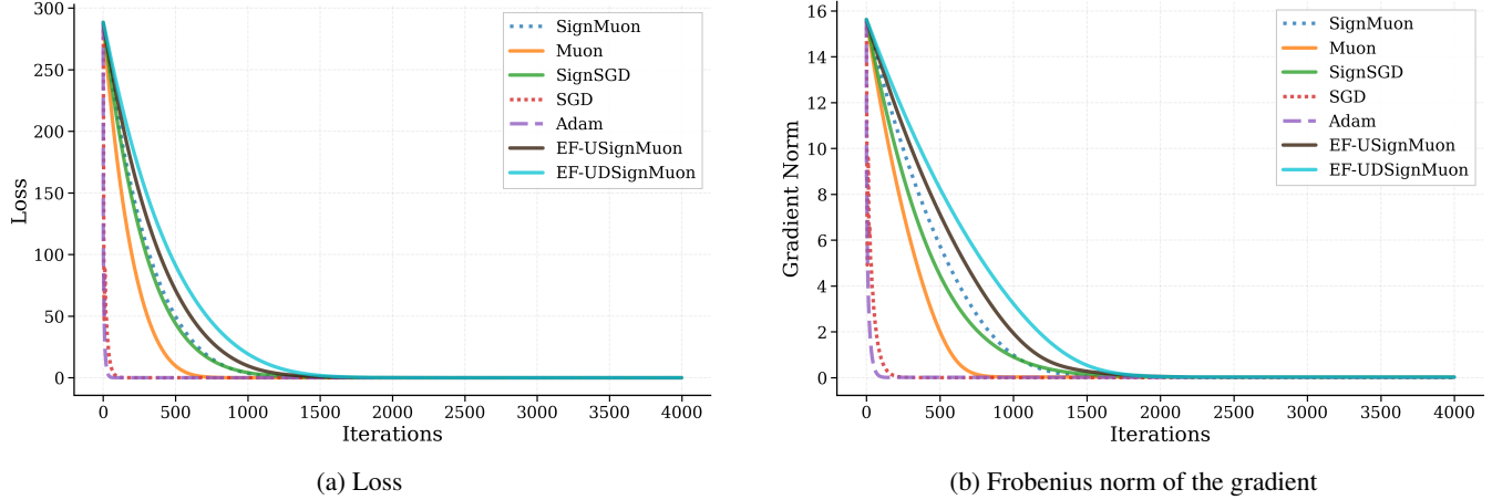
Figure 7: Smooth convex problem (Equation 47 for 500 \times 500 ).
