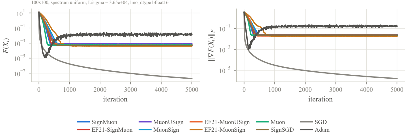
Figure A2: Trajectories at the optima of Table A3, one curve per method, mean over three problem draws. Every normalized method flattens onto a plateau within a few hundred iterations and stays there for the remaining 4000-odd, which is the behaviour the accuracy-floor reading of the fixed-target criterion predicts and the reason the crossing time is a ranking of floors. SGD, whose step vanishes with the gradient, is the one curve still descending at T_{\max} ; Adam’s oscillates around its own floor rather than settling onto it. This is the current-protocol counterpart of Figure A5, at m = n = 100 rather than 500, and the iteration counts of the two are not comparable.
