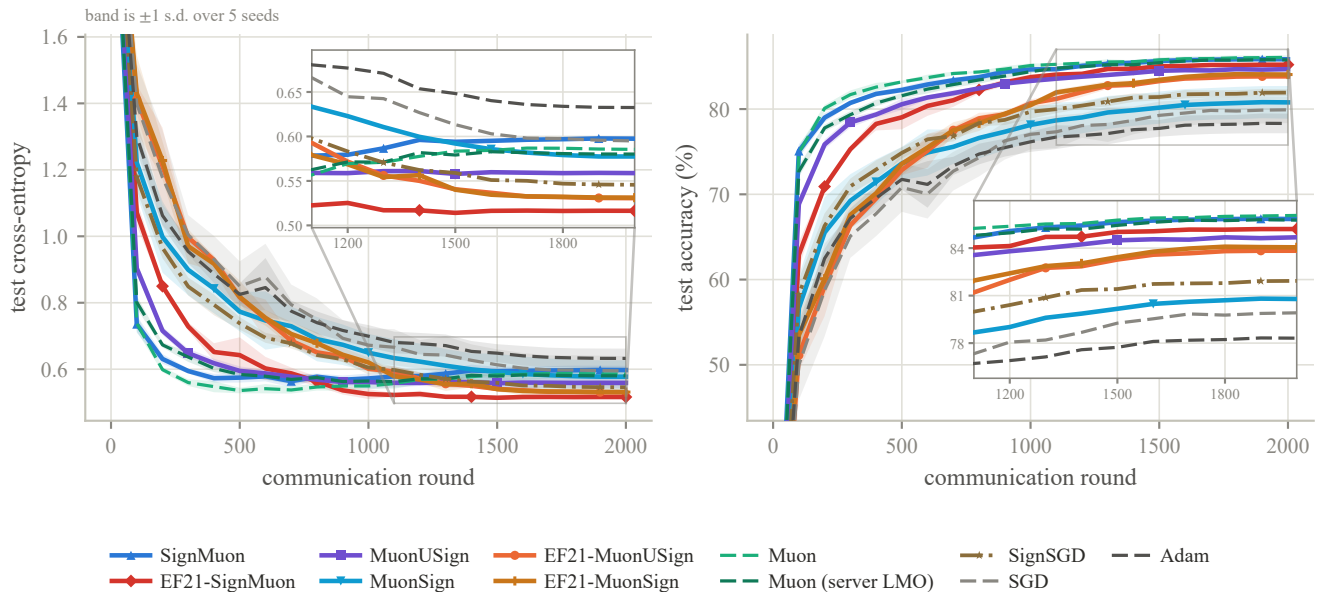
Figure A9: CIFAR-10 federated learning on CNN2 at N = 11 clients and batch 192 per client: test cross-entropy (left) and test accuracy (right) against communication round. Each curve is the mean over five seeds and the band is \pm 1 sample standard deviation across them; all methods are evaluated on the exact server model \mathbf{X}_t . Both axes are clipped to exclude round 0, which is the untrained model and identical for every method. Line style carries the method’s role — solid for the one-bit methods, dashed for the uncompressed references, dash-dot for SignSGD — so that hue is not the only channel separating eleven curves; markers are spaced apart per method for the same reason. The insets magnify the final 45% of rounds, where every number in Table 2 is read and where the curves lie within a line width of one another; bands are omitted inside them, since at that zoom they overlap into a single wash. Eleven methods are drawn, one more than Table 2, the extra being the server-side-LMO Muon control.
