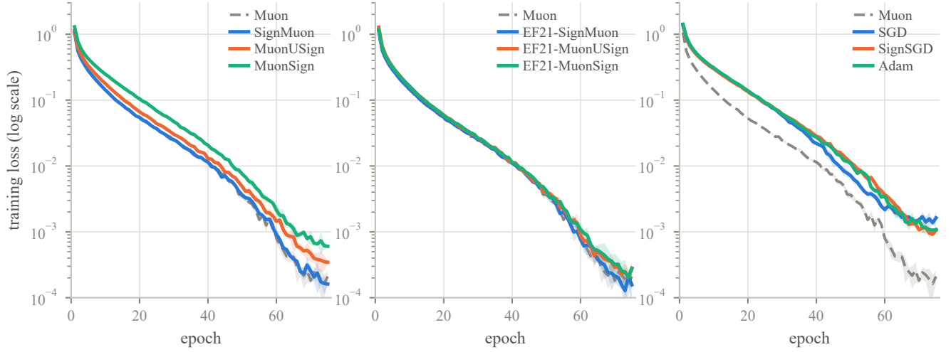
Figure A7: Training loss (log scale), grouped as in Figure 2 and over the same runs. Within a panel the methods are hard to separate (every one of them falls to 10^{-3} or below, and they differ mainly in how early), which is why the body figure carries the accuracy alone. What the loss does show is the gap between families: in the right panel Muon reaches a given loss some fifteen epochs ahead of SGD, SignSGD and Adam and ends nearly an order of magnitude lower, while in the left panel SignMuon tracks Muon and the sign-before and both-sides orderings trail it, in the same order as their accuracies.
