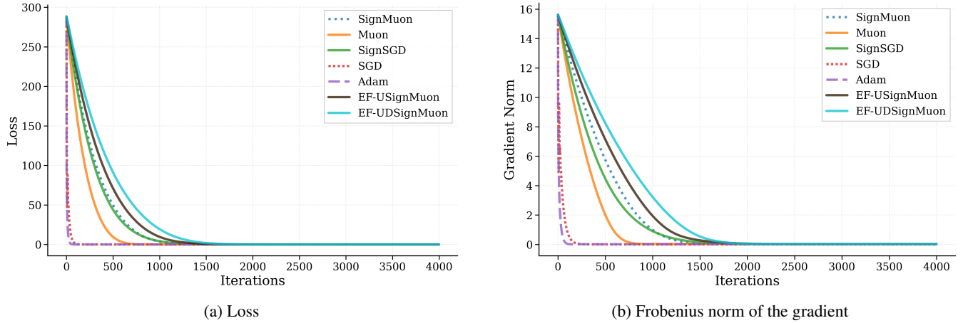
Figure A5: Smooth convex problem (Equation 30 for 500 \times 500 ).
