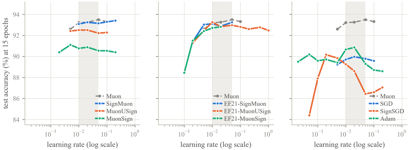
Figure A8: Learning-rate sweep at 15 epochs on the tuning split, grouped as in Figure 2, with Muon repeated as the gray dashed reference. The shaded band marks \eta_0 \in [0.01, 0.05] , the range every method except EF21-MuonSign was swept over and therefore the only range-matched comparison: within it the LMO methods vary by 0.16–0.42 points (Muon itself, 0.28, is no flatter than the sign variants), while Adam varies by 1.57 and SignSGD by 2.82. The robustness belongs to the LMO, and taking the sign of its output does not cost it.
