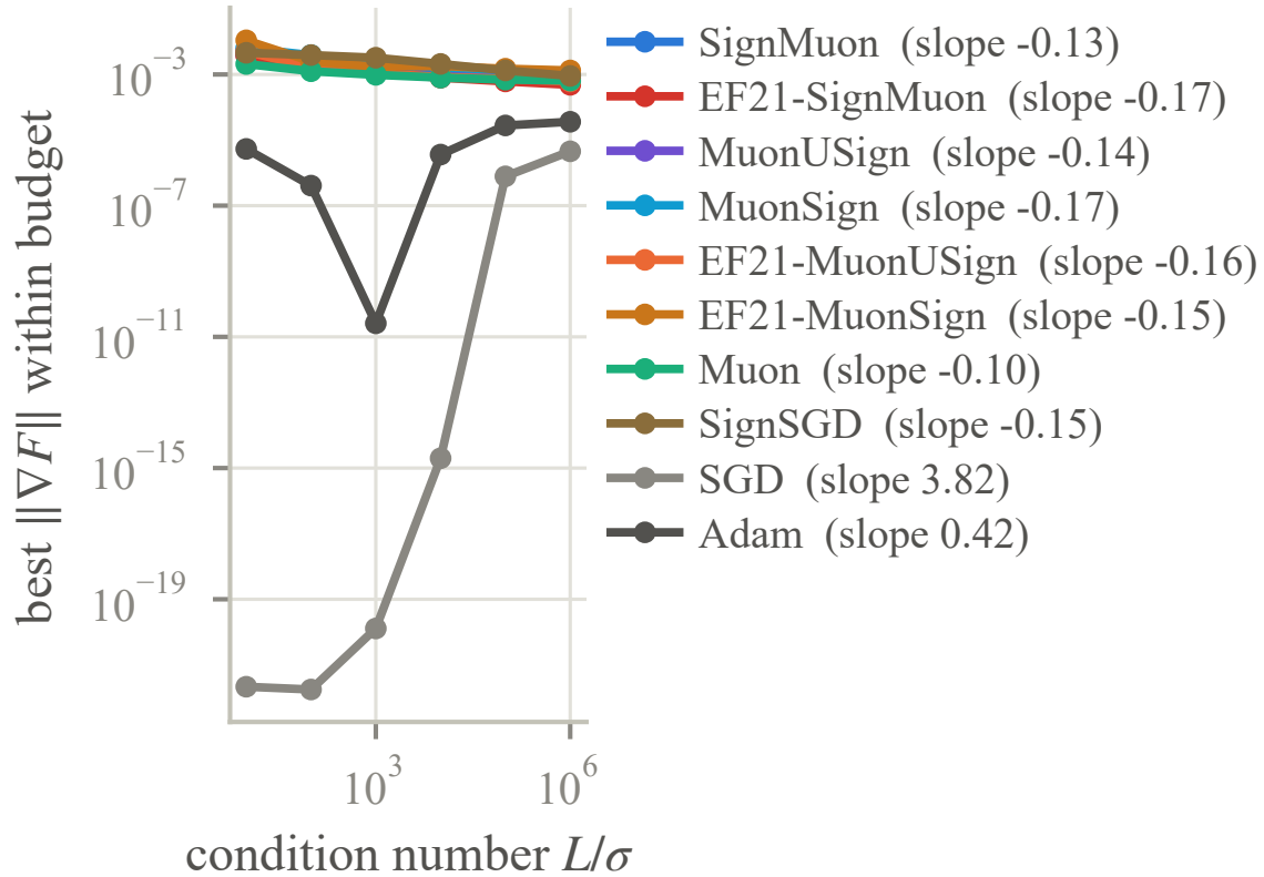
Figure A4: Best \|\nabla F\| within the budget against the condition number L/\sigma , tuned at each point. The eight norm-fixed methods lie in a band an order of magnitude wide and essentially flat; SGD and Adam are the two that resolve the sweep at all.
