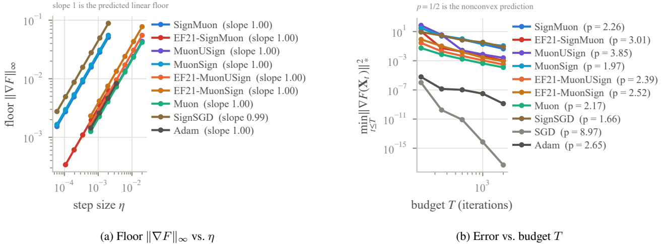
Figure A3: Log-log fits behind Table A5. Left: the accuracy floor of a constant step. The lines are parallel because every exponent is 1, and the two clusters are the two windows of \eta swept, one per step length. EF21-SignMuon is in the left cluster although its step has length \sqrt{r} , because it was swept over the sign family’s window; that is the misassignment the protocol paragraph reports, and it displaces the line along \eta without changing its slope. Right: best error at each tuned budget, in the norm dual to each method’s own LMO ball, so the curves are comparable within a family and not across one.
