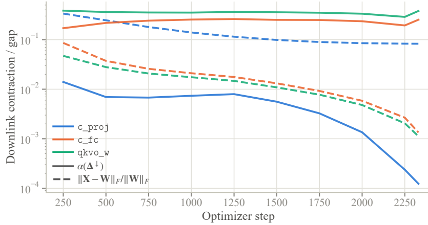
Figure A11: The downlink measurement for EF21-MuonSign, per layer type: the contraction \alpha(\Delta^\downarrow) the scaled sign actually achieves (solid) and the resulting server/broadcast gap \|\mathbf{X}_t - \mathbf{W}_t\|_F / \|\mathbf{W}_t\|_F (dashed). On the zero-initialized c_{\text{proj}} the contraction is two orders of magnitude below the rest from step 250 on and falls a further two by the end, and the gap stops decreasing near 10^{-1} ; every other layer type contracts at \Theta(10^{-1}) and closes its gap by 6–64 \times over the run, ending below 10^{-2} . This is Remark 3 measured.
