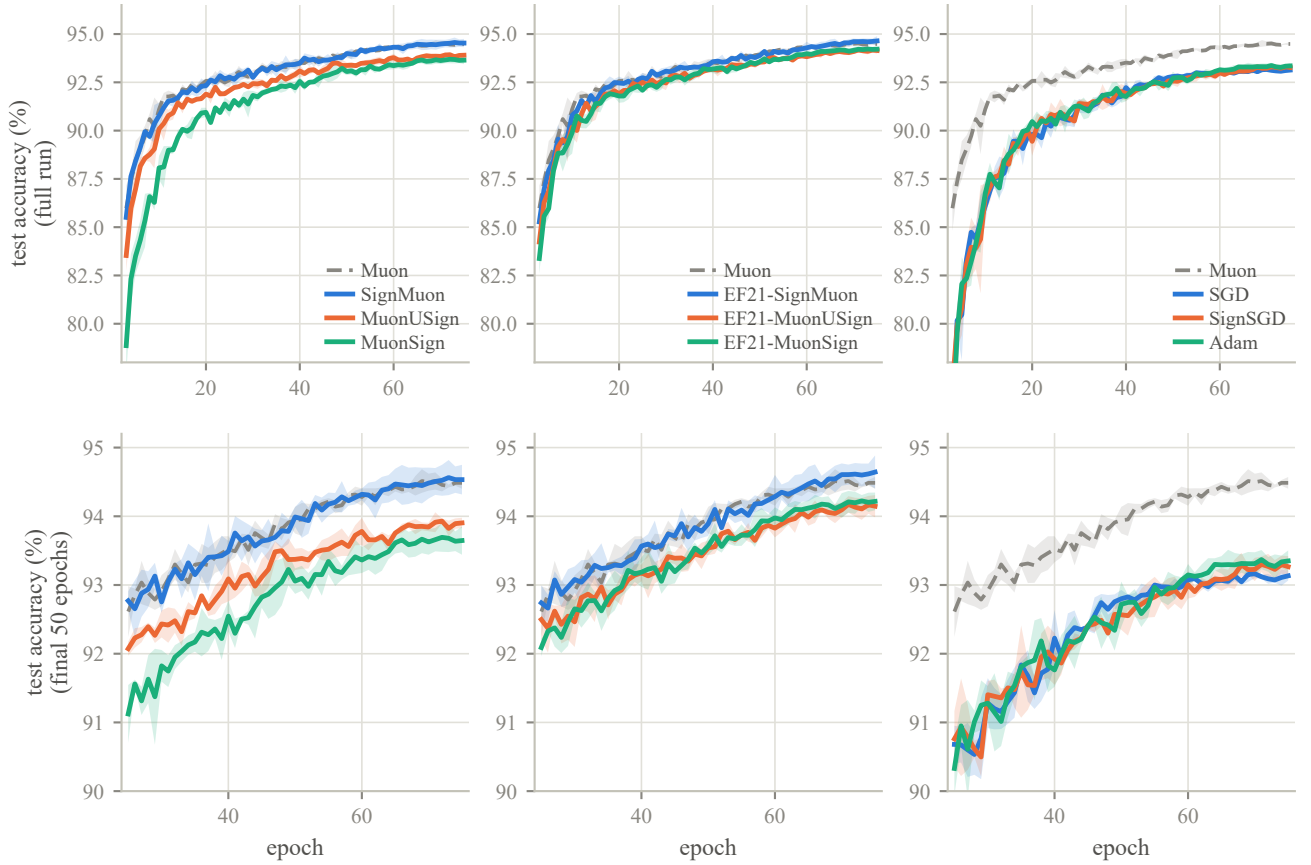
Figure A6: Test accuracy over the whole run (top row) and from epoch 25 (bottom row), the same data at two scales, grouped as in Figure 2. Bands are \pm 1 standard deviation over three seeds; Muon is the gray dashed reference in every panel. Series are labelled at the right of each panel.
