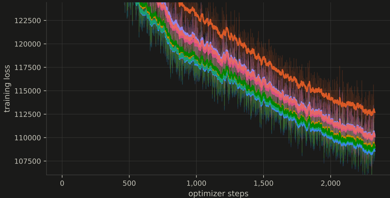
NanoGPT speedrun (record #40): training loss vs steps
