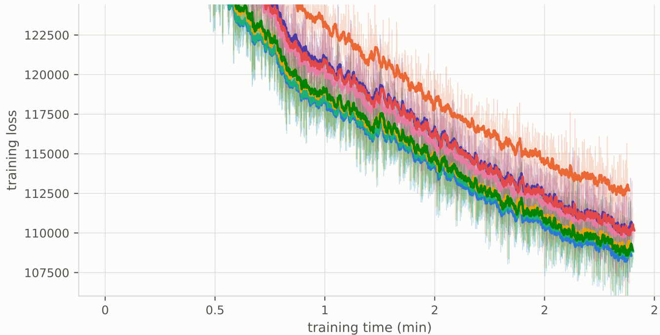
NanoGPT speedrun (record #40): training loss vs wall-clock
