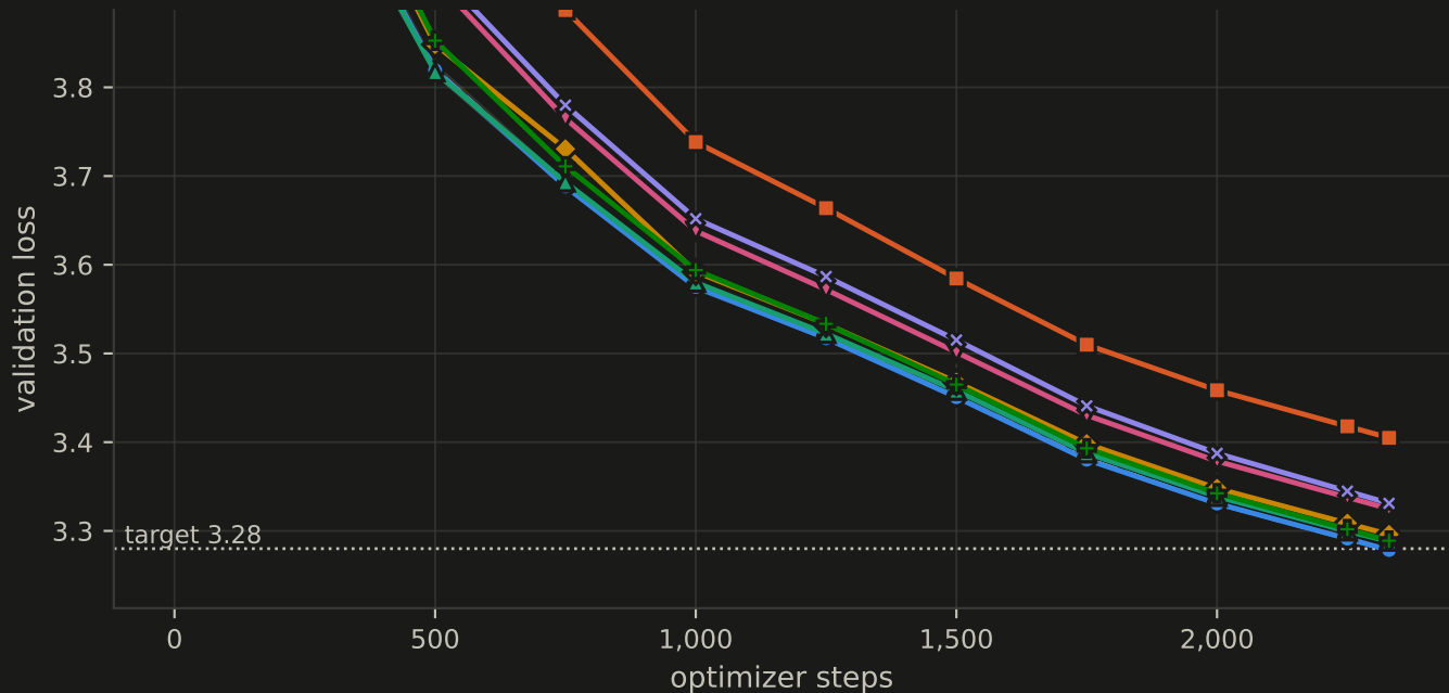
NanoGPT speedrun (record #40): validation loss vs steps
