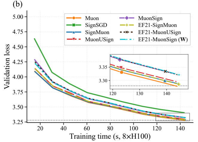
Figure 13: NanoGPT, supporting curves. (a) Training loss against optimizer step (EMA-smoothed; the logged quantity is a per-rank sum over 32,768 tokens, divided out here). (b) Validation loss against the speedrun clock, which excludes validation and compilation. Insets magnify the boxed tails, as in Figure 3. The ordering is the same on both axes: no method pays a measurable wall-clock premium for its compressor or its error-feedback buffers. Note in (a) that EF21-MuonSign’s training loss – taken at \mathbf{W} – is healthy throughout, which is what isolates its validation gap to the \mathbf{X} -tracking rather than to training.
