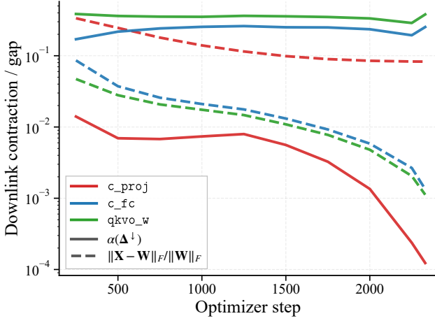
Figure 14: The downlink measurement for EF21-MuonSign, per layer type: the contraction \alpha(\Delta^\dagger) the scaled sign actually achieves (solid) and the resulting server/broadcast gap \|\mathbf{X}_t - \mathbf{W}_t\|_F / \|\mathbf{W}_t\|_F (dashed). On the zero-initialized c_proj the contraction is two orders of magnitude below the rest from step 250 on and falls a further two by the end, and the gap stalls near 10^{-1} ; every other layer type contracts at \Theta(10^{-1}) and closes its gap by 6–64 \times over the run, ending below 10^{-2} . This is Remark 3 measured.
