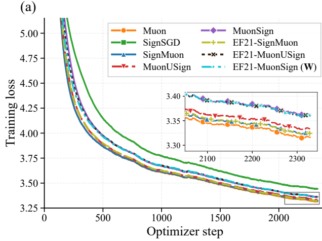
Figure 13: NanoGPT, supporting curves. (a) Training loss against optimizer step (EMA-smoothed; the logged quantity is a per-rank sum over 32,768 tokens, divided out here). (b) Validation loss against the speedrun clock, which excludes validation and compilation. Insets magnify the boxed tails, as in Figure 3. The ordering is the same on both axes: no method pays a measurable wall-clock premium for its compressor or its error-feedback buffers. Note in (a) that EF21-MuonSign’s training loss – taken at \mathbf{W} – is healthy throughout, which is what isolates its validation gap to the \mathbf{X} -tracking rather than to training.
