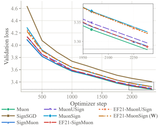
Figure 3: NanoGPT speedrun, 8 \times H100 : validation loss against optimizer step, single seed; dotted line is the speedrun target 3.28. EF21-MuonSign is drawn at its broadcast model W . The inset magnifies the boxed tail, where SignSGD is above the range shown; exact values are in Table 3.
