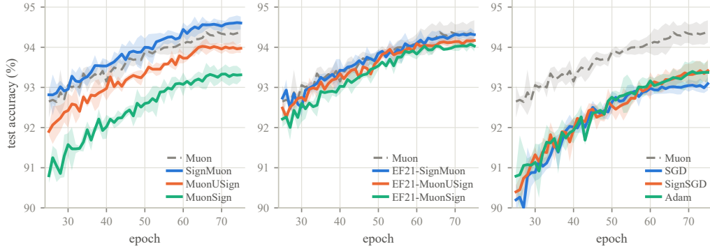
Figure 2: Centralized ResNet-18 on CIFAR-10: test accuracy at the \eta_0 selected for each method, from epoch 25 (Table 2). Panels group the sign placements, the EF21 variants and the baselines; Muon is the gray dashed reference, bands \pm 1 s.d. over three seeds. The numbers are Table 2, Appendix A.4.
