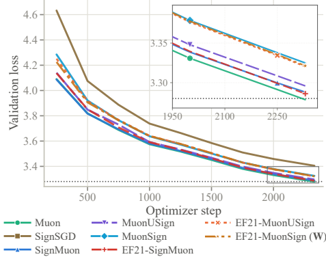
Figure 3: NanoGPT speedrun, 8 \times H100 : validation loss against optimizer step, one run per method; dotted is the target 3.28, and EF21-MuonSign is drawn at its broadcast model \mathbf{W} . The inset magnifies the boxed tail, where SignSGD lies above the range shown.
