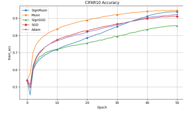
(b) Train Accuracy
