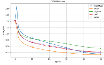
(a) Train Loss
