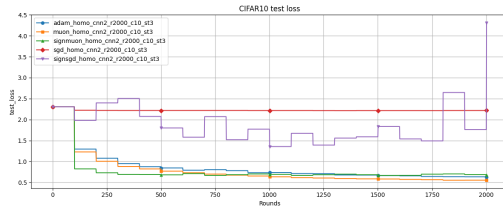
(a) Test Loss
