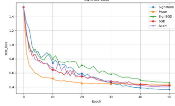
(c) Test Loss
