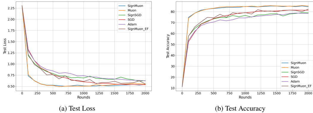
Figure 7: CIFAR-10 Federated Learning. Experiment 3: Comparison of Optimization Algorithms with (N = 10) Clients.
