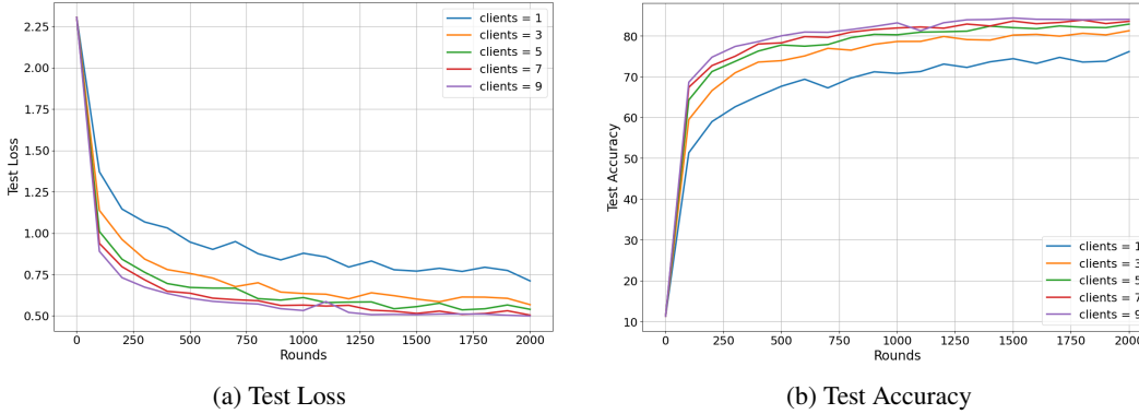
Figure 5: CIFAR-10 Federated Learning. Experiment 1. Scalability of the SignMuon Algorithm.
