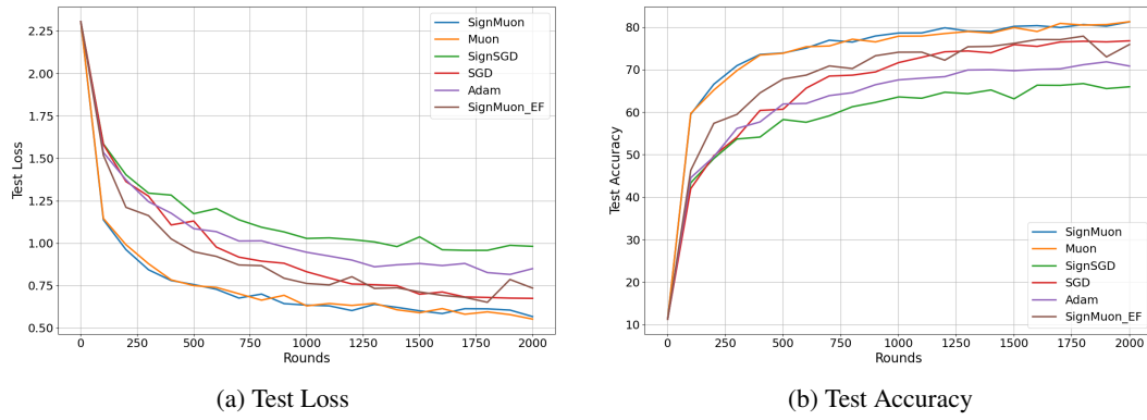
Figure 6: CIFAR-10 Federated Learning. Experiment 2: Comparison of Optimization Algorithms with (N = 3) Clients.
