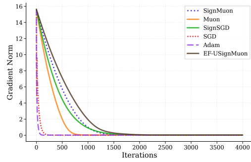
(b) Frobenius norm of the gradient
