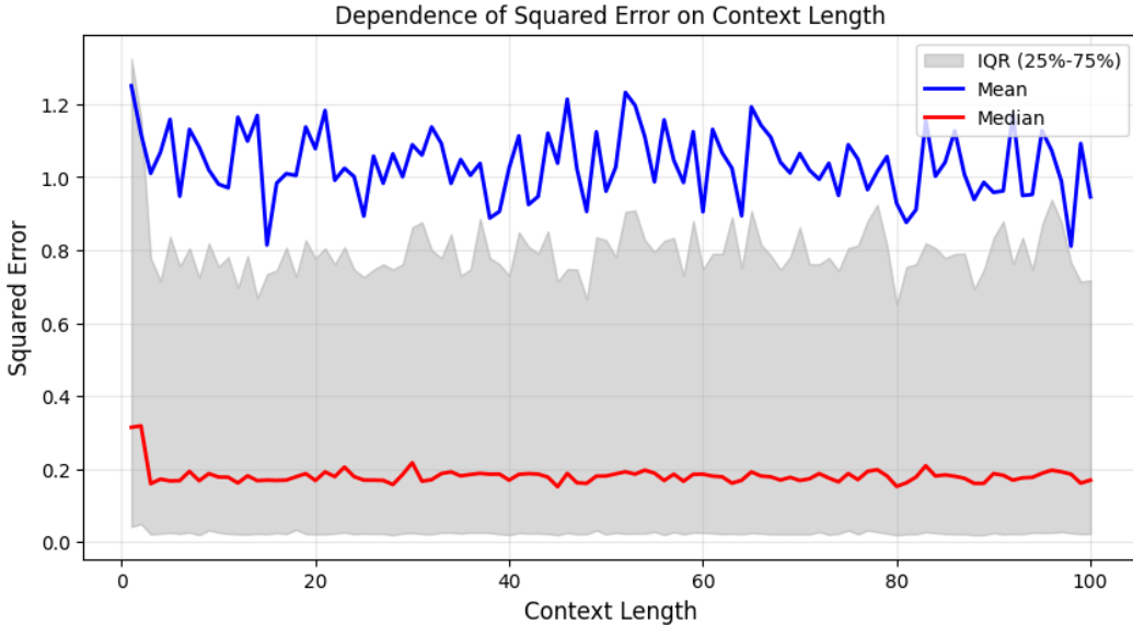
Figure 12: Dependence of Squared Error on context length.
