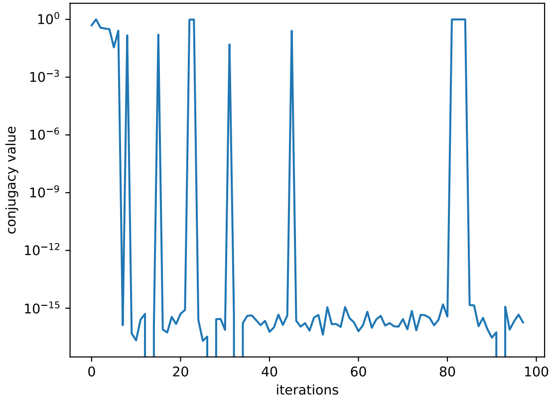
Conjugacy value by iterations
