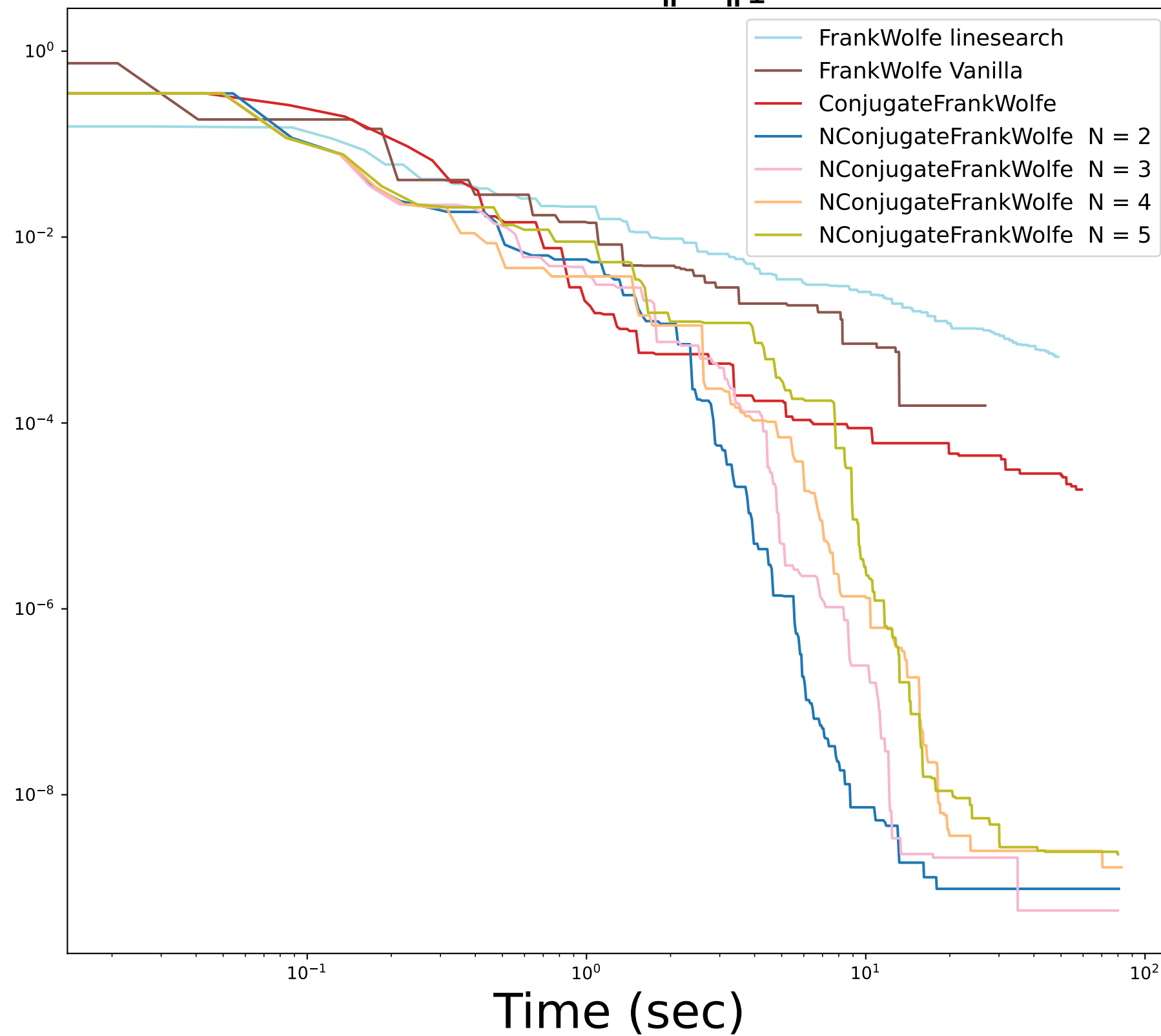
Constraints \|w\|_1 < 5
